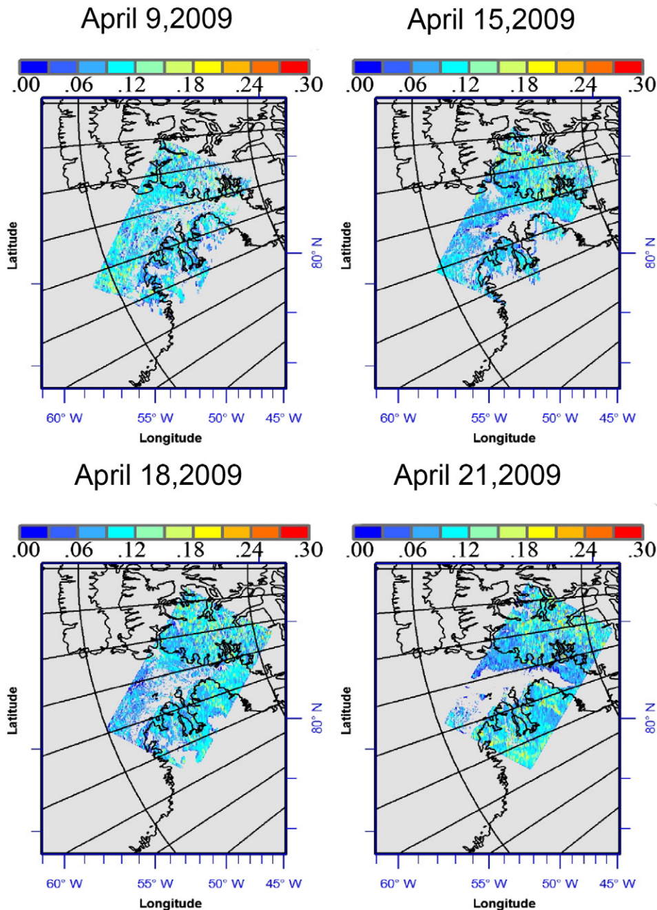
Fig. 25. Maps of aerosol optical thickness \tau(0.55 \mu\text{m}) retrieved from AATSR data taken with 1 \text{ km} \times 1 \text{ km} resolution on 9, 15, 18, and 21 April, 2009, over snow-covered surfaces in west Greenland using the method of Mei et al. (2013b).
