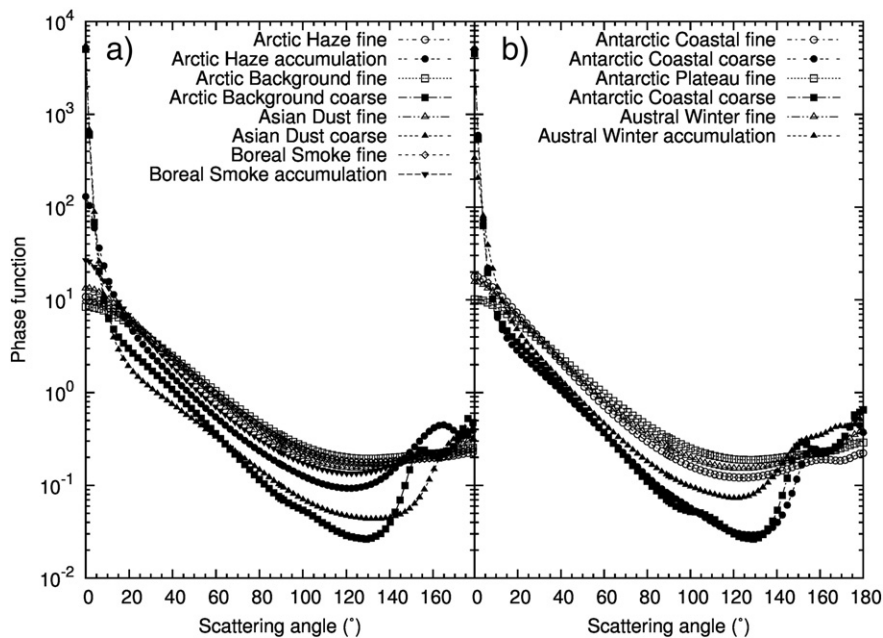
Fig. 26. Angular distribution curves of phase function P(\theta) as a function of the scattering angle \theta for the 8 unimodal Arctic aerosol extinction models (left) and the 6 unimodal Antarctic aerosol extinction models defined in Table 5.
