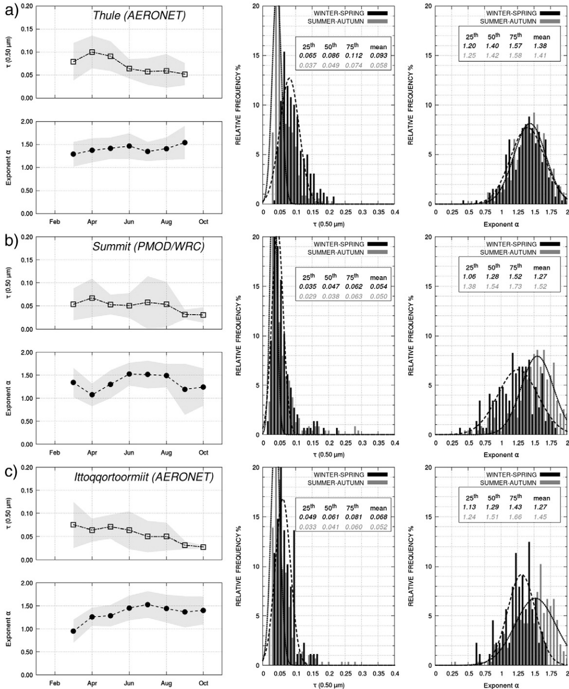
Fig. 5. As in Fig. 3, for the for the multi-year sun-photometer measurements of aerosol optical thickness \tau(0.50 \mu\text{m}) and exponent \alpha conducted at: (a) Thule (North-western Greenland) by NASA/GSFC (USA) over the period from March 2007 to September 2012, using an AERONET Cimel CE-318 sun-photometer having the spectral characteristics reported in Table 1; (b) Summit (Central Greenland) by PMOD/WRC (Switzerland) from January 2001 to October 2011, using a PFR (No. N34) sun-photometer of the GAW-PFR network, having the spectral characteristics given in Table 1; and (c) Ittoqqortoormiit (Eastern Greenland) by NASA/GSFC (USA) over the period from May 2010 to October 2013, using an AERONET Cimel CE-318 sun-photometer having the spectral characteristics reported in Table 1.
