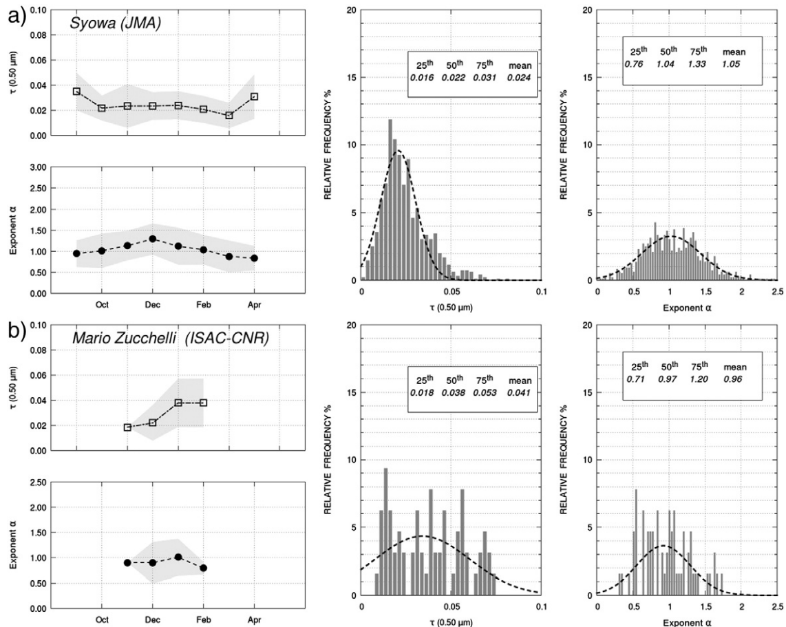
Fig. 11. As in Fig. 3, for sun-photometer measurements of aerosol optical thickness \tau(0.50 \mu\text{m}) and exponent \alpha conducted at the Antarctic sites of: (a) Syowa (East Ongul Island, Lützow-Holm Bay) over the period from January 2000 to December 2011 by the Office of Antarctic Observation (Japan Meteorological Agency, Tokyo, Japan), using the EKO MS-110 sun-photometer, having the spectral characteristics given in Table 2; and (b) Mario Zucchelli on the Terra Nova Bay (Ross Sea, Victoria Land) during the austral summer periods of 2001/2002 and 2005/2006 by ISAC-CNR (Bologna, Italy), using the PREDE POM-01 L and the ASP-15WL sun-photometers, having the spectral characteristics given in Table 2.
