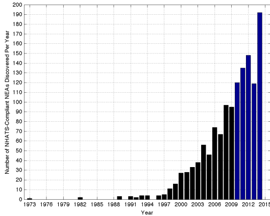
Figure 1: The number of accessible (NHATS-compliant) NEAs discovered each year since the first one (Anteros) was discovered in 1973.
