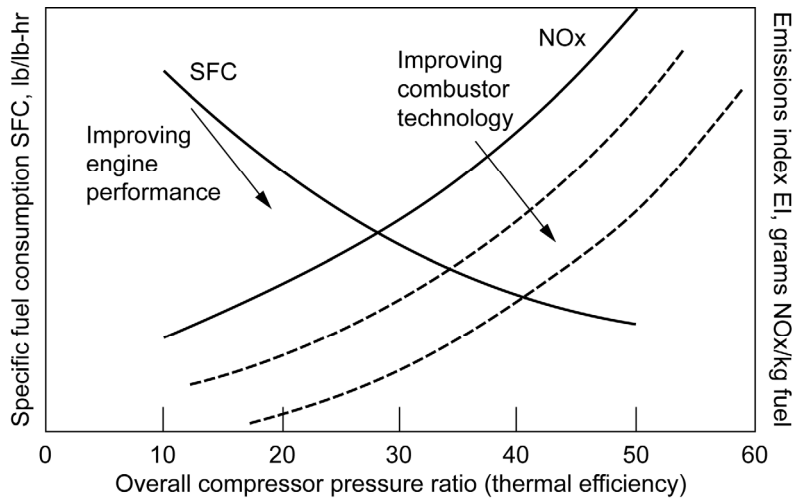
Figure 2.—Impact of overall engine cycle pressure ratio on NOx formation. Increasing pressure ratio reduces fuel consumption at the cost of producing NOx. However, the NOx curve can be lowered by improving the combustor and its sub-component technologies.
