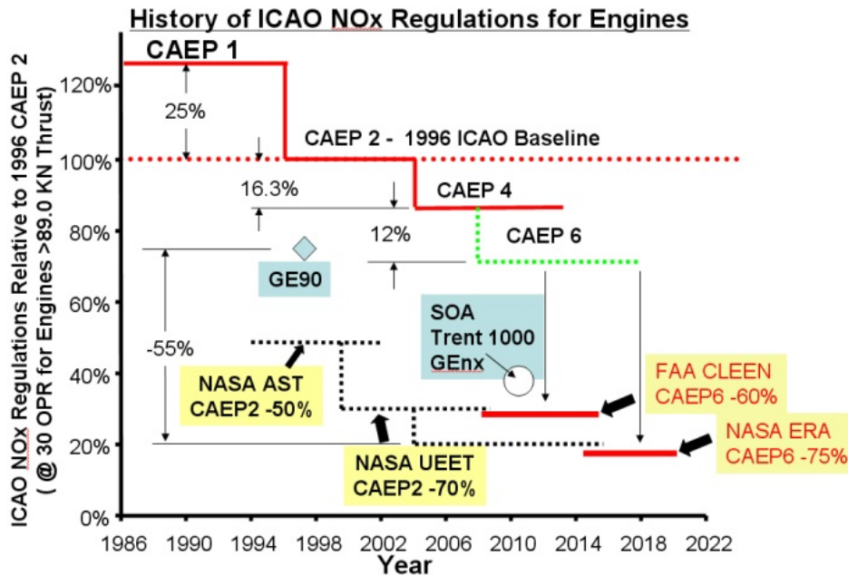
Figure 3.—Historical trends of ICAO LTO NOx limit and NASA program goals.
