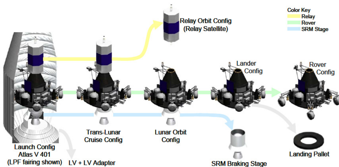
Figure 14.—Rover Configuration at Different Mission Stages (Ref. 8).
