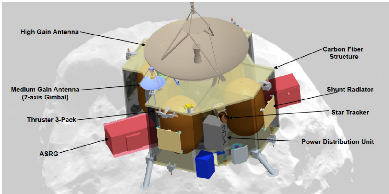
Figure 18.—Ilion Spacecraft/Lander Concept Illustration (Ref. 10).
