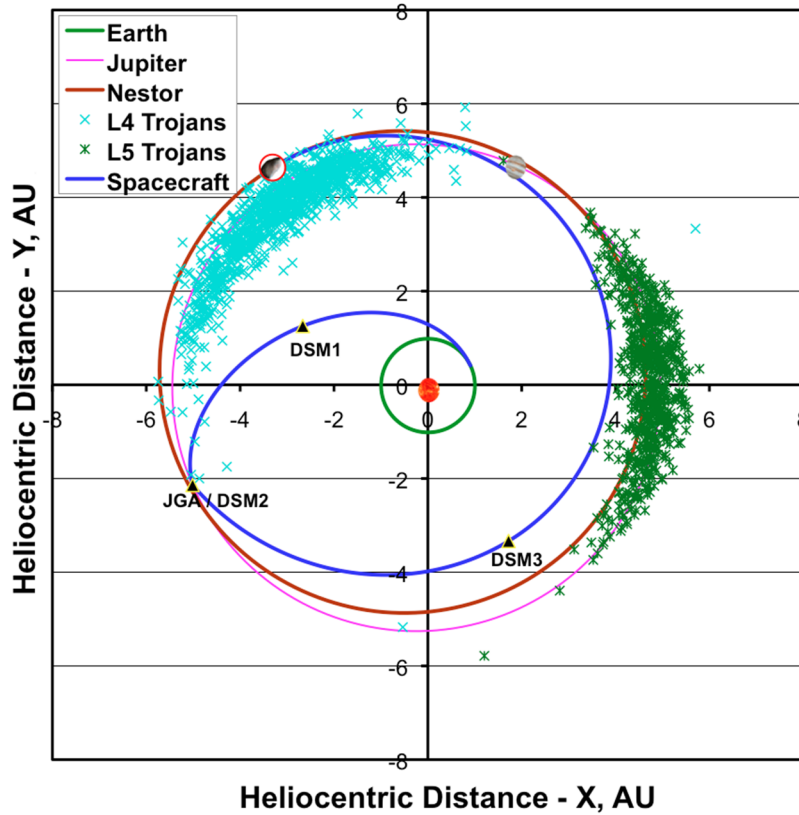
Figure 19.—Iliion Orbital Trajectory (Ref. 10).
