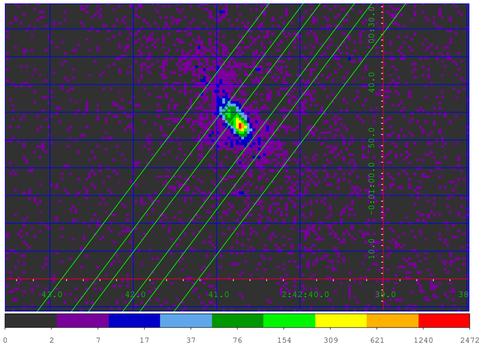
Fig. 6.— Zero order image with positions of extraction regions shown. Lines corresponds to standard extraction region (4.8 arcsec width) plus half and double size regions as discussed in text. Only heg arm is shown for clarity.
