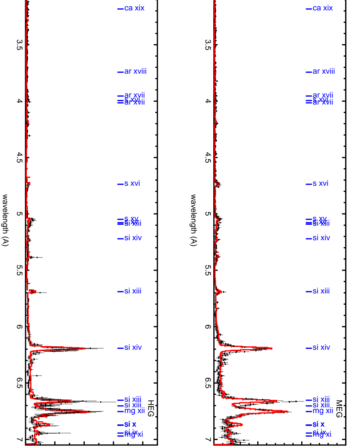
Fig. 4. Spectrum showing fits to table model described in the text. Vertical axis is counts s^{-1}Hz^{-1} scaled according to the maximum flux in the panel.
