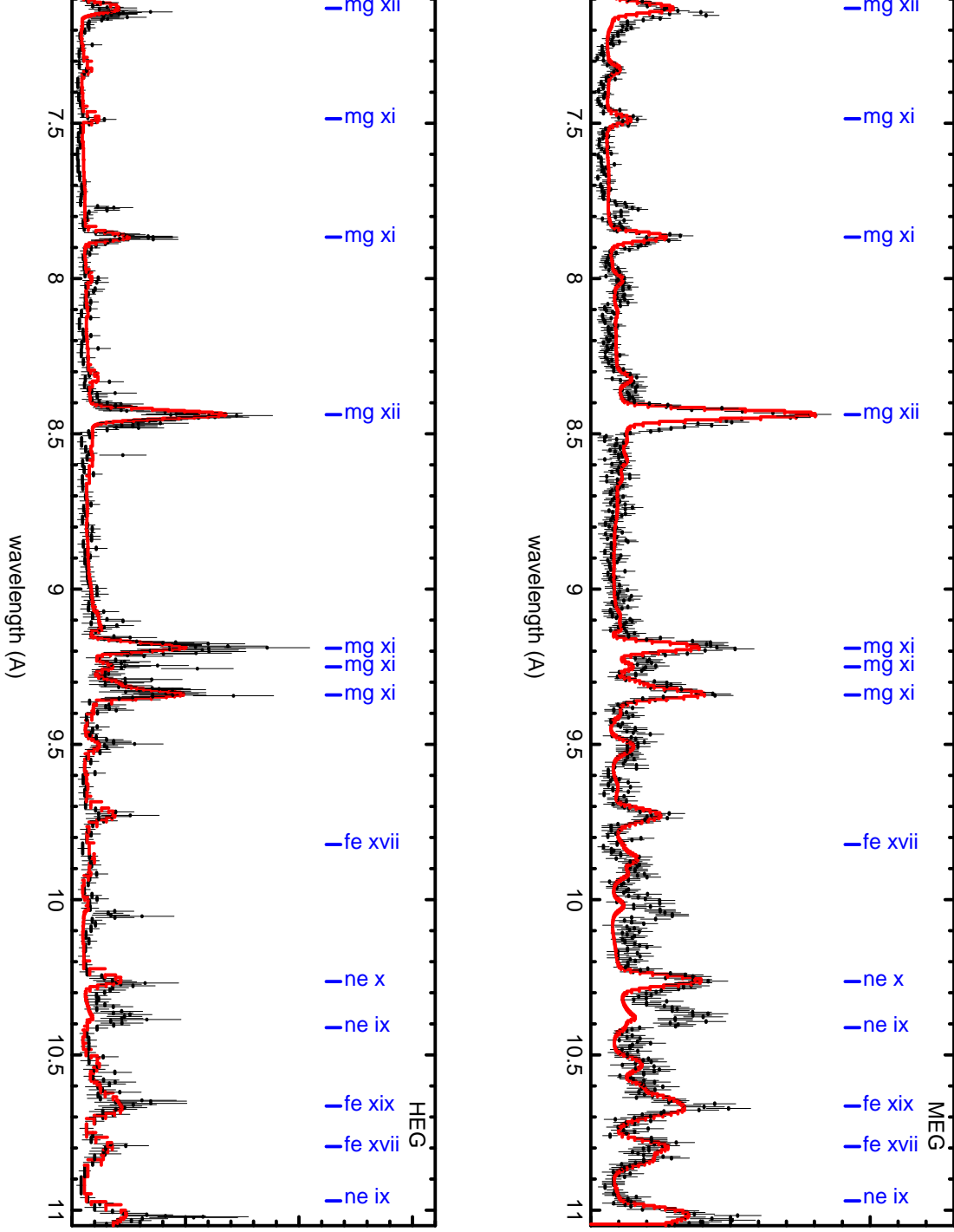
Fig. 3.— Spectrum showing fits to table model described in the text. Vertical axis is counts s^{-1}Hz^{-1} scaled according to the maximum flux in the panel.
