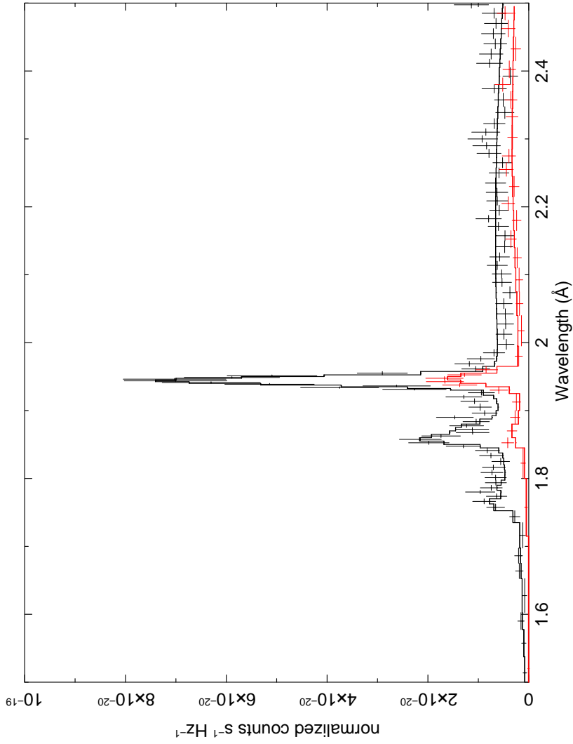
Fig. 10.— Fe K line region. Lines are apparent from near-neutral Fe near 1.95 \text{ \AA} , He-line near 1.85 \text{ \AA} and H-like near 1.75 \text{ \AA} . The model consists of components with and without radiative excitation from the analytic model described in section 3, plus power law continuum.
