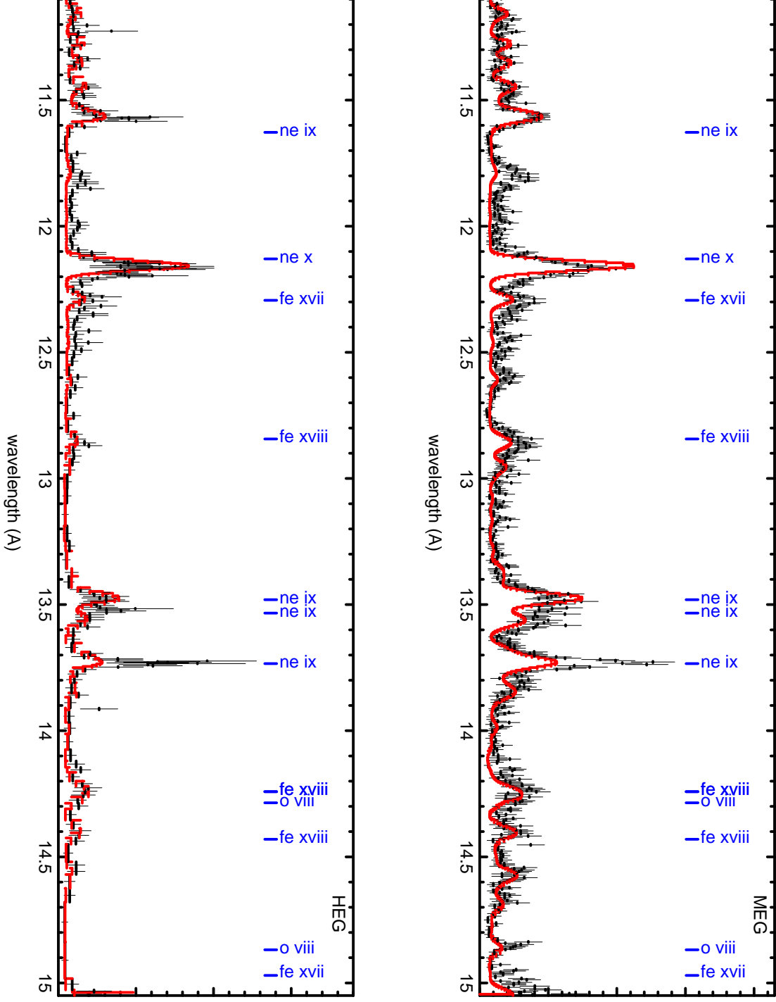
Fig. 2. Spectrum showing fits to table model described in the text. Vertical axis is counts s^{-1}Hz^{-1} scaled according to the maximum flux in the panel.
