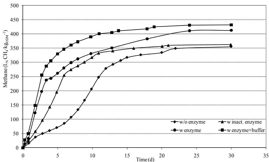
Figure 5 Methane production from rye grain silage, without enzyme application and with application of inactivated and active enzyme, the latter without and with buffer (Values shown here are means of three replicates, for variance coefficient and significance cf. Table 3)
