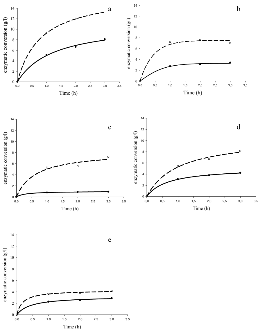
Figure 2 Effect of enzyme concentration on sugar formation of different feedstock a) rye grain silage, b) maize silage, c) grass silage, d) feed residue, e) solid cattle manure; solid line 0.02 \text{ g enzyme} \cdot \text{g}_{\text{ODM}}^{-1} feedstock, dashed line 0.04 \text{ g enzyme} \cdot \text{g}_{\text{ODM}}^{-1} feedstock. (Values shown here are means of three replicates with variance coefficient less than 0.094 )
