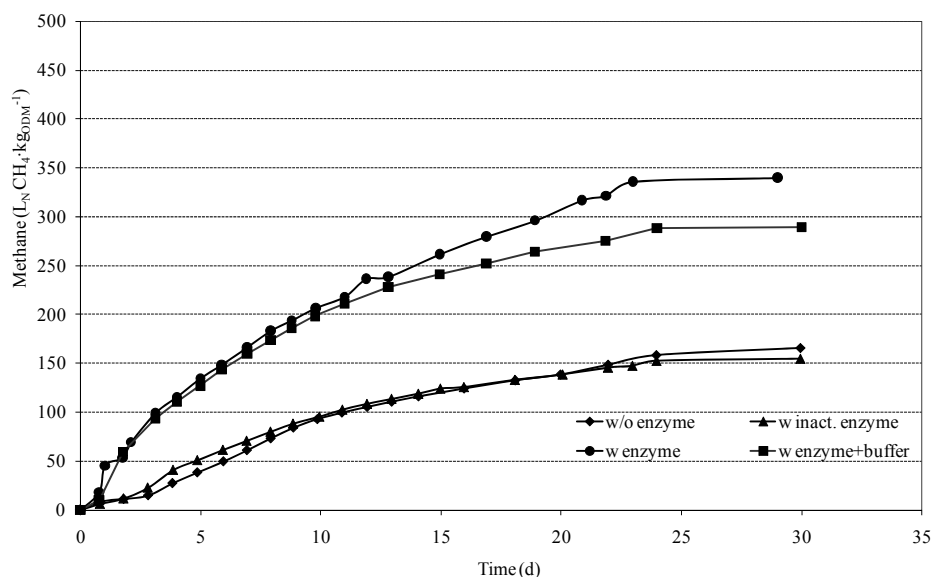
Figure 9 Methane production from solid cattle manure, without enzyme application and with application of inactivated and active enzyme, the latter without and with buffer (Values shown here are means of three replicates, for variance coefficient and significance cf. Table 3)
