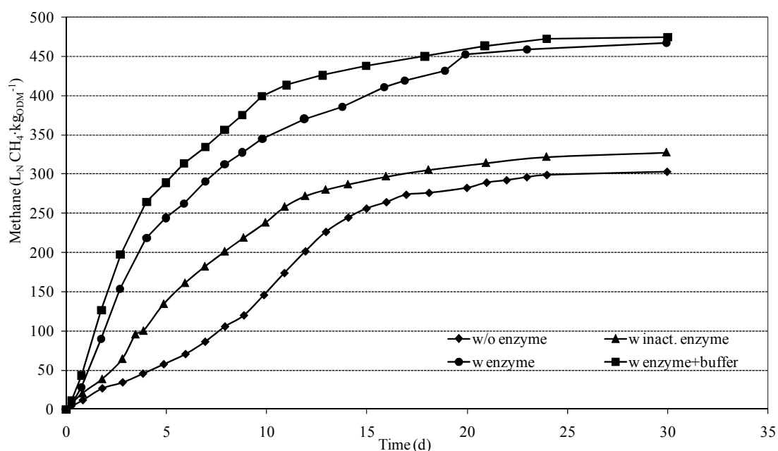
Figure 8 Methane production from feed residue silage, without enzyme application and with application of inactivated and active enzyme, the latter without and with buffer (Values shown here are means of three replicates, for variance coefficient and significance cf. Table 3)
