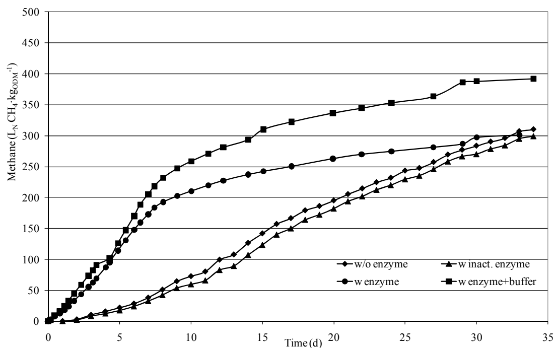
Figure 7 Methane production from grass silage, without enzyme application and with application of inactivated and active enzyme, the latter without and with buffer (Values shown here are means of three replicates, for variance coefficient and significance cf. Table 3)
