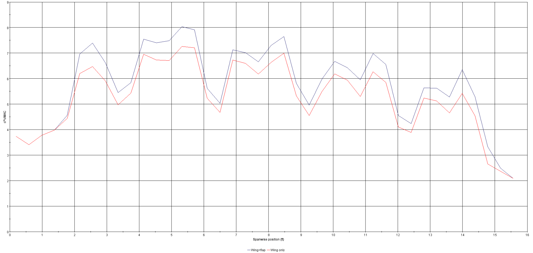
Lift distribution, 10°, 300 hp, 40° flaps, 61 KEAS
