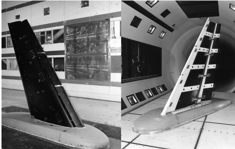
Figure-2.2.1: NASA Trap Wing Geometry in the wind tunnel (Image reference: AIAA HLPW-1)
