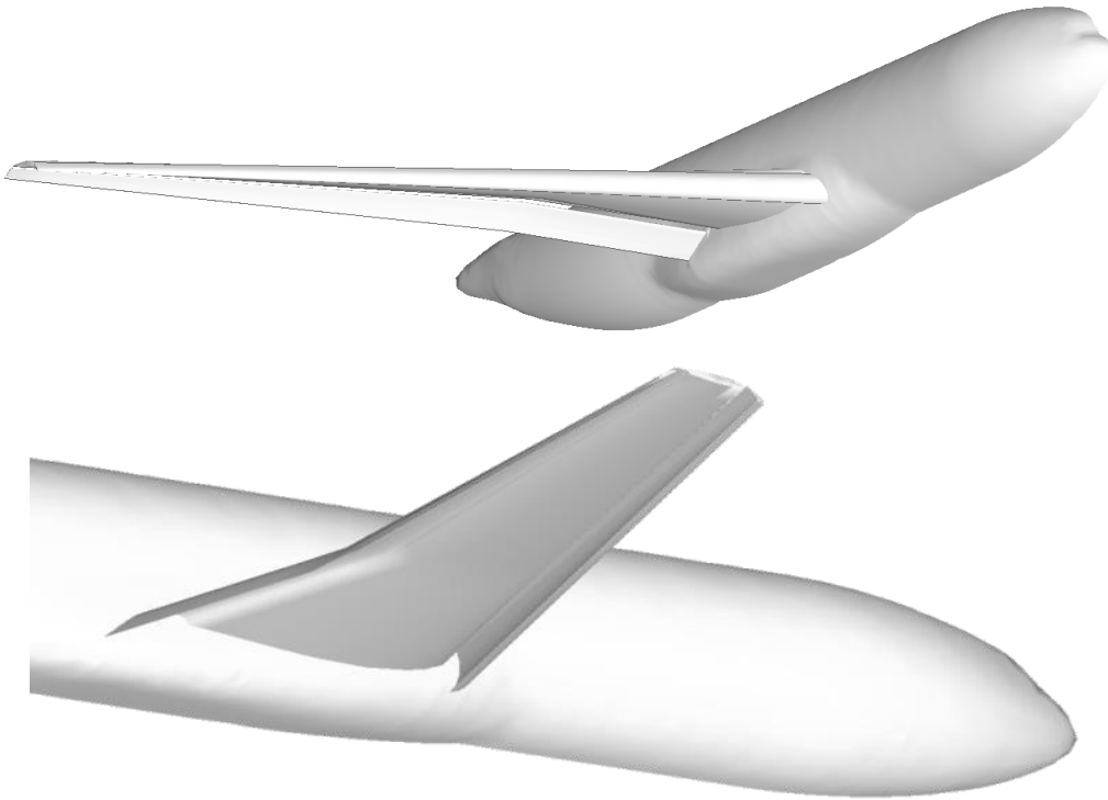
Figure-2.3.1: The DLR-F11 geometry as imported into the FlightStream™ solver
