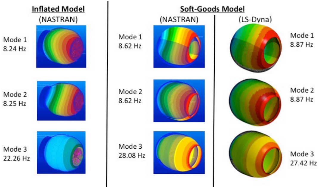
Figure 5. Comparison of first 3 free vibration modes.
