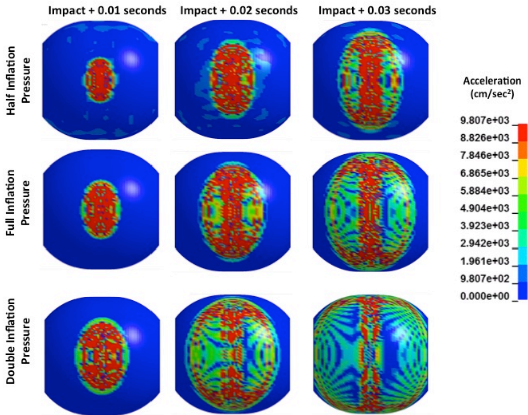
Figure 6. Effect of Inflation pressure on acceleration wave for Soft-Goods Model.
