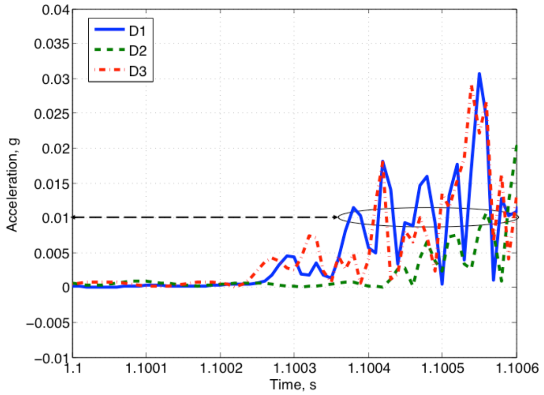
Figure 12. Sample time histories for bulkhead impulse at the DIDS bulkhead sensor locations.
