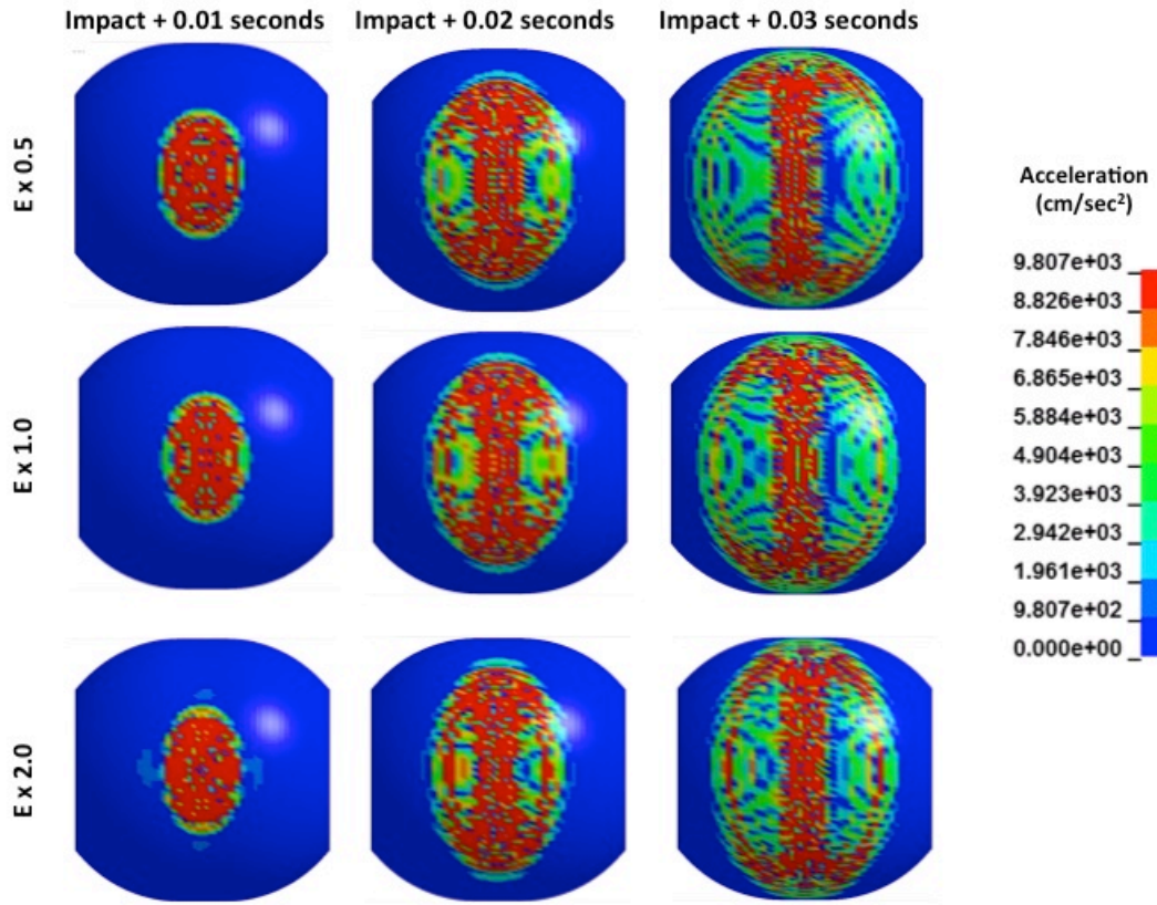
Figure 7. Effect of elastic modulus on acceleration response for Soft-Goods Model.
