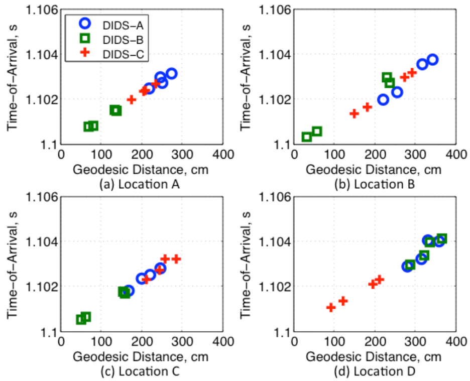
Figure 11. Correlation of impulse Time-of-Arrival with geodesic distance for Soft-Goods excitations and responses.
