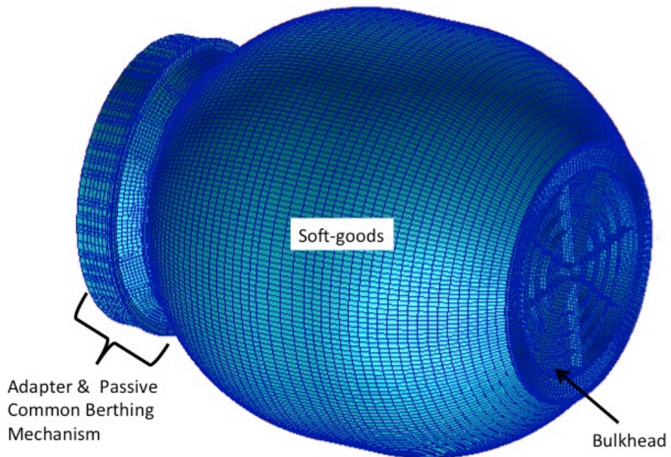
Figure 2. NASTRAN Inflated Model.
