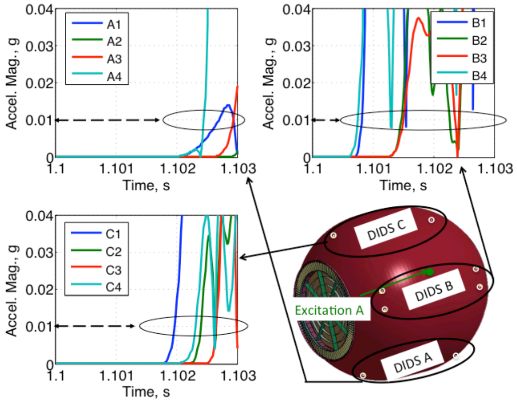
Figure 10. Sample time histories for Soft-Goods impulse at the Soft-Goods DIDS sensor locations.
