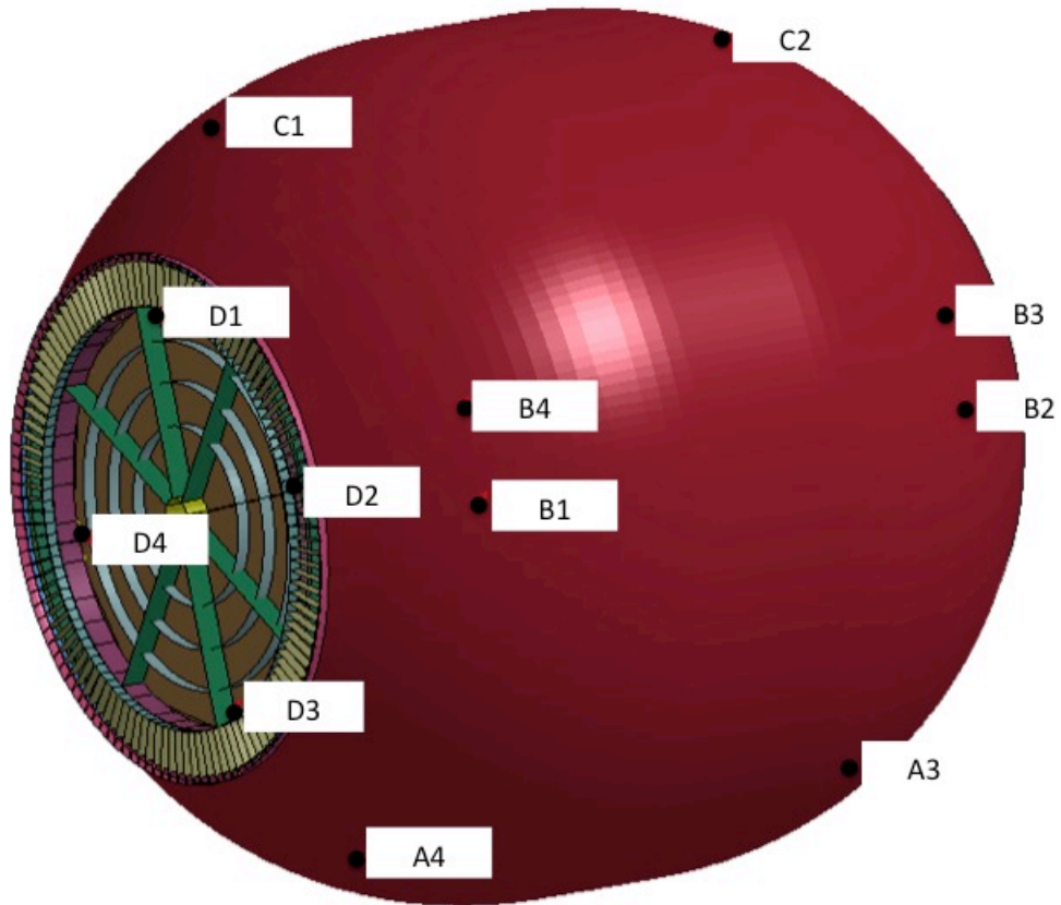
Figure 8. DIDS accelerometer locations.
