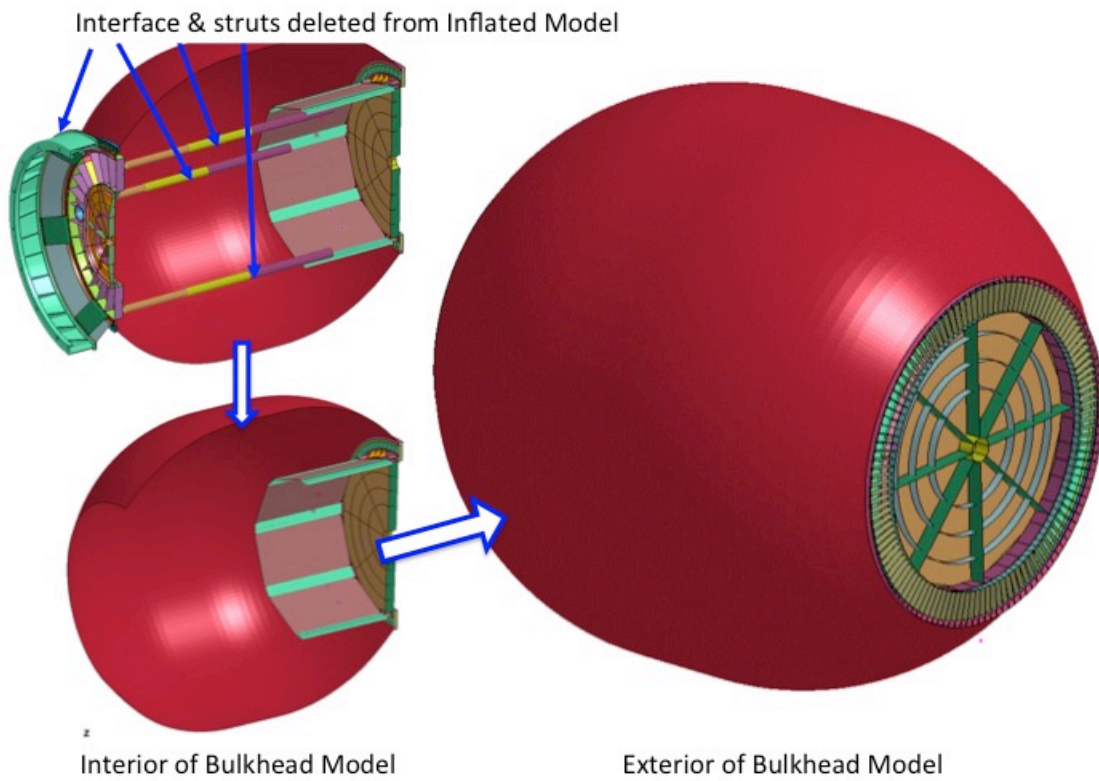
Figure 4. Schematic of Bulkhead Model.
