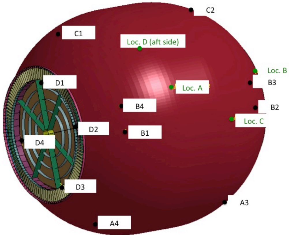
Figure 9. DIDS acceleration locations along with nodal excitation locations shown in green.
