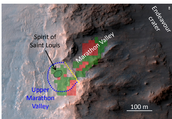
Figure 1. HiRISE image overlain with CRISM detections of smectite (red - strong; green - less strong).
