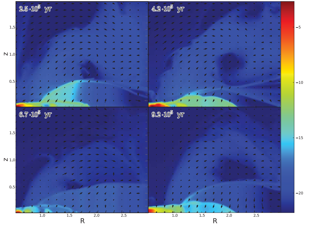
Fig. 6.— Color plot of the density, \log \rho in (g \text{ cm}^{-3}) for the model with L = 0.1 L_{\text{edd}} shown at different times given in years. Axes: horizontal: z : distance from equatorial plane in parsecs; R : distance from the BH in parsecs;
