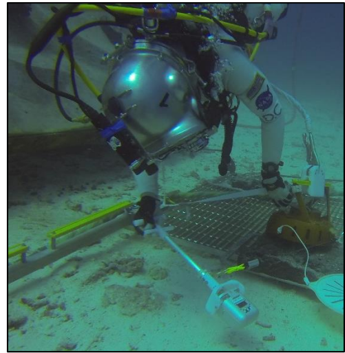
Figure 3. Float Collection at NEEMO 20 using a Microspine for Body Stabilization
