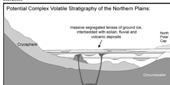
Figure. 2. Potential for the sequestration of a potentially large initial surface inventory of water and ice by the deposition of subsequent mantles of volcanic ash, lavas and eolian and fluvial sediments.
