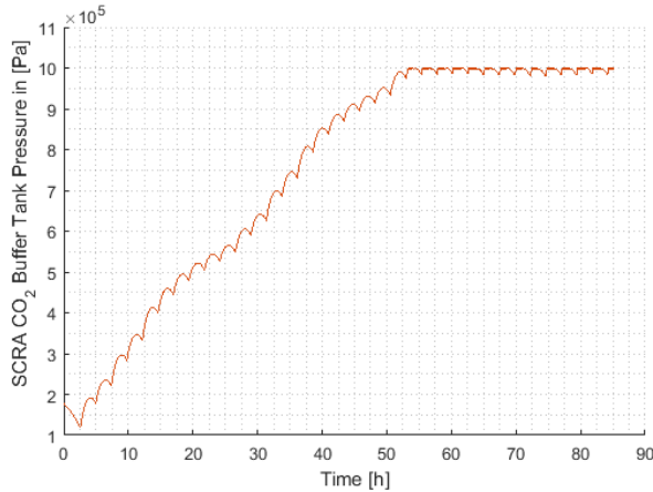
Figure 7. CO 2 Supply to US Sabatier System.
