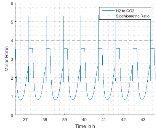
Figure 8. CO 2 Supply to ACLS Sabatier System.
