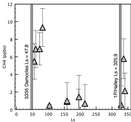
Figure 2: Methane detections by the Mars Science Laboratory rover with cometary encounters from Table 2 inserted. Data adapted from [6]. Note the appearance of methane shortly after Mars' interactions with the orbits of 5335 Damocles and 1P/Halley, both of which are large cometary bodies
