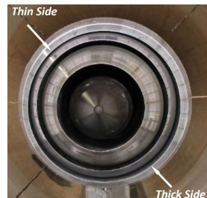
Figure 5. Offset nozzles installed in HFJER and NATR viewed from downstream.
