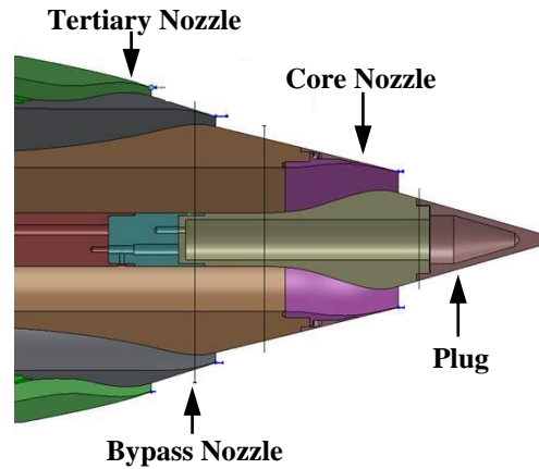
Figure 2. The axisymmetric-nozzle system used in the three-stream experiments.
