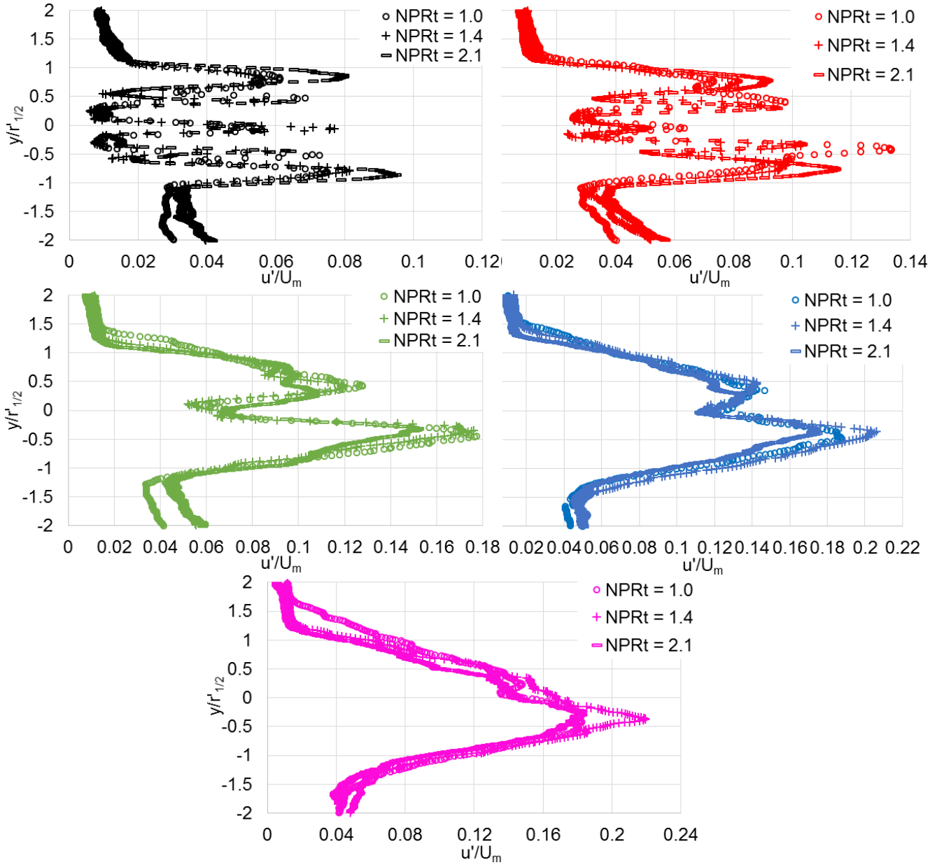
Figure 32. The normalized turbulence intensity for the heated three-stream jets at the indicated NPRt. The data were acquired with A_b/A_c = 1 and at M_{fj} = 0.0 . Black, red, green, blue, and magenta indicate x/D_{eqA} = 0 , x/D_{eqA} = 2 , x/D_{eqA} = 4 , x/D_{eqA} = 6 , and x/D_{eqA} = 8 , respectively.
