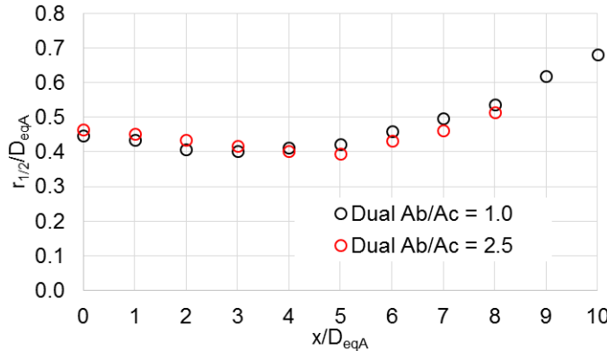
Figure 23. The half-velocity radii for the heated jet conditions and the indicated dual-stream jets. The data were acquired with the A_t/A_c = 1.0 and M_{fj} = 0.3 .
