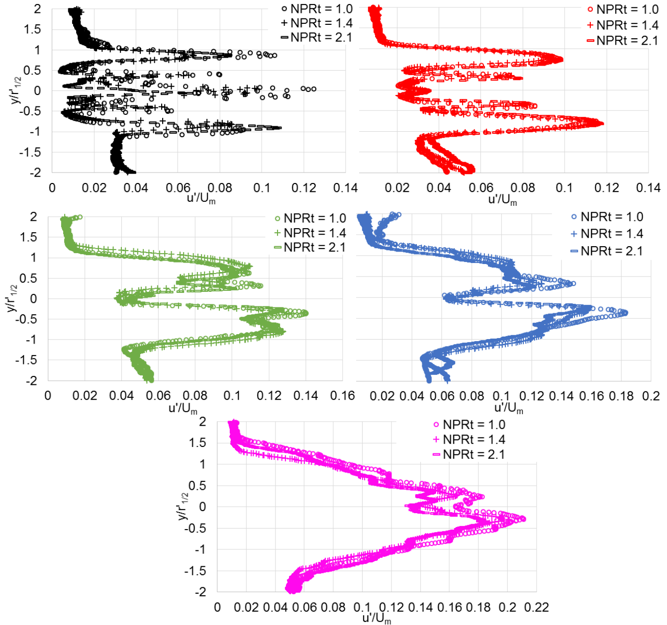
Figure 34. The turbulence intensity for the heated three-stream jets at the indicated NPR_t . The data were acquired with A_b/A_c = 2.5 and at M_{fj} = 0.3 . Black, red, green, blue, and magenta indicate x/D_{eqA} = 0 , x/D_{eqA} = 2 , x/D_{eqA} = 4 , x/D_{eqA} = 5 , and x/D_{eqA} = 7 , respectively.
