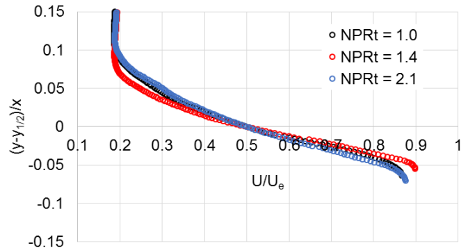
Figure 21. The velocity at the indicated cross-stream planes for the heated dual- and three-stream jets. The data were acquired for M_{fj} = 0.0 and with the A_b/A_c = A_t/A_c = 1.0 nozzle system.
