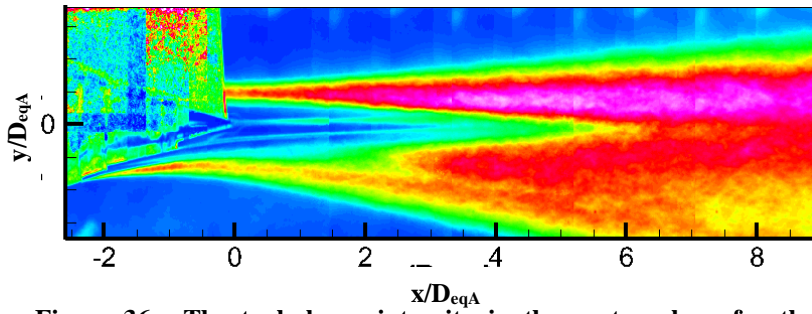
Figure 36. The turbulence intensity in the center plane for the unheated offset three-stream jet with NPR_t = 1.8 and M_{fj} = 0.0 . The legend is the same as that in Fig. 31.
