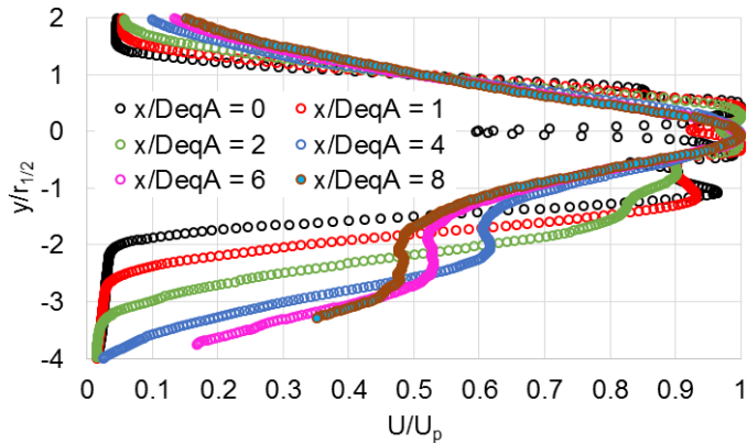
Figure 26. The velocities at the indicated cross-stream plane for the unheated three-stream jet with the tertiary offset. The data are for NPR_t = 1.8 and M_{fj} = 0.0 and were acquired with the A_b/A_c = 1.0 nozzle system.
