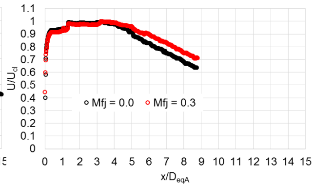
Figure 10. The centerline velocities for NPR_c = 1.8 , NPR_b = 1.8 , NPR_t = 1.4 , NTR_c = 3.0 and the indicated free jet Mach numbers.
