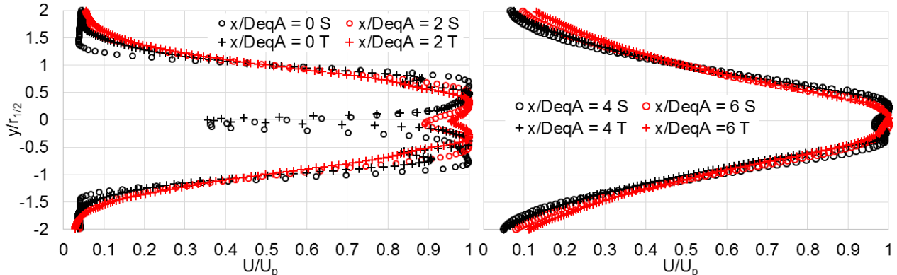
Figure 17. The velocity at the indicated cross-stream planes for the unheated single-stream (S) and three-stream (T) jets. The data were acquired at M_{fj} = 0.0 with the A_b/A_c = A_t/A_c = 1.0 nozzle system.
