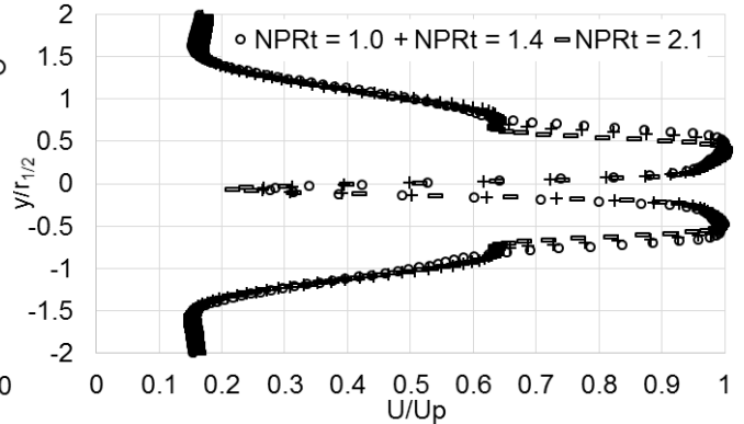
Figure 24. The mean velocity for the heated dual- and three-stream jets at x/D_{eqA} = 0 . The data were acquired with the A_b/A_c = 1.0 and A_t/A_c = 0.6 nozzle system and for M_{fj} = 0.3 .
