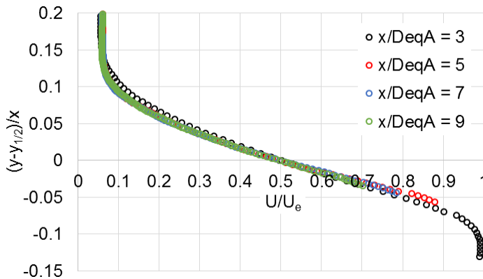
Figure 15. The velocity at the indicated cross-stream planes for the unheated single-stream jet and M_{fj} = 0.0 .
