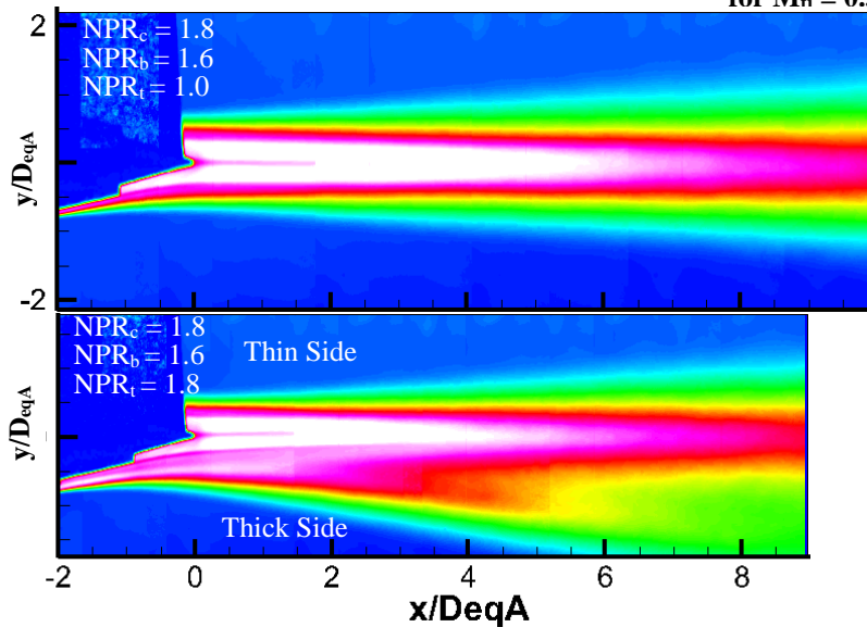
Figure 25. The mean velocity in the center plane for the unheated dual-stream (top) and three-stream offset (bottom) jets. The conditions are indicated on the contour plots. The legend is the same as that in Fig. 4 with U_c equal to the core exit velocity. The data were acquired for M_{fj} = 0.0 .
