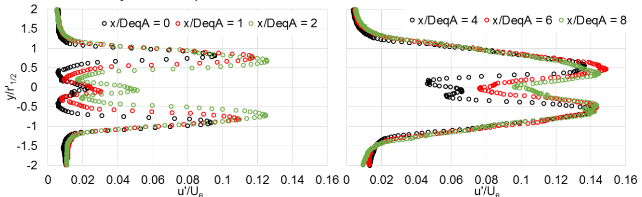
Figure 29. The turbulence intensity at the indicated cross-stream planes for the unheated simulated single-stream jet with A_b/A_c = 1.0 and M_{fj} = 0.0 .
