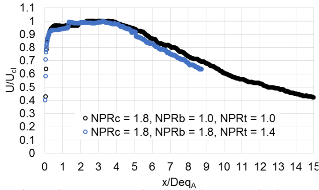
Figure 9. The centerline velocities at the indicated nozzle pressure ratios and NTR_c = 3.0 . The data were acquired for M_{fj} = 0.0 .
