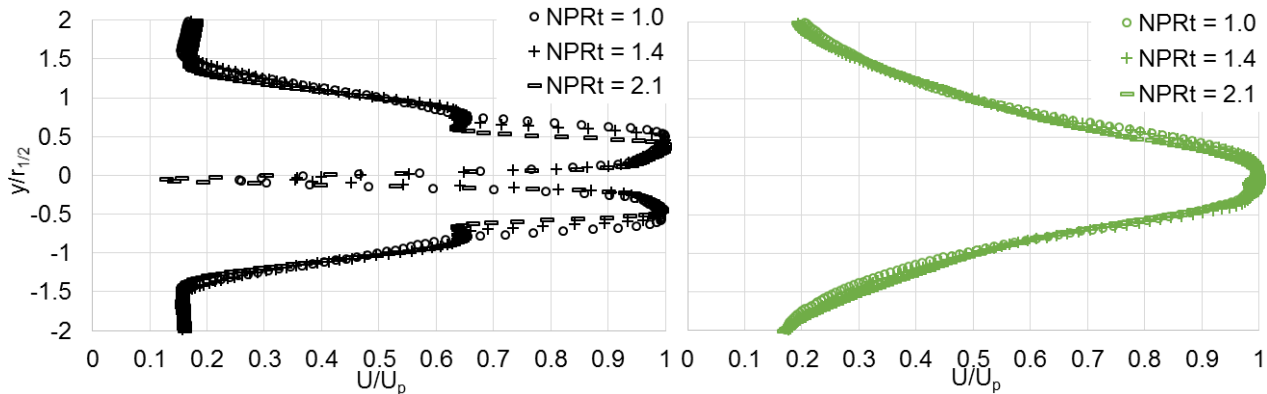
Figure 19. The velocity for the heated jet conditions and A_b/A_c = A_t/A_c = 1 . The black and green are for x/D_{eqA} = 0 and 4, respectively. The data are for M_{fj} = 0.3 .
