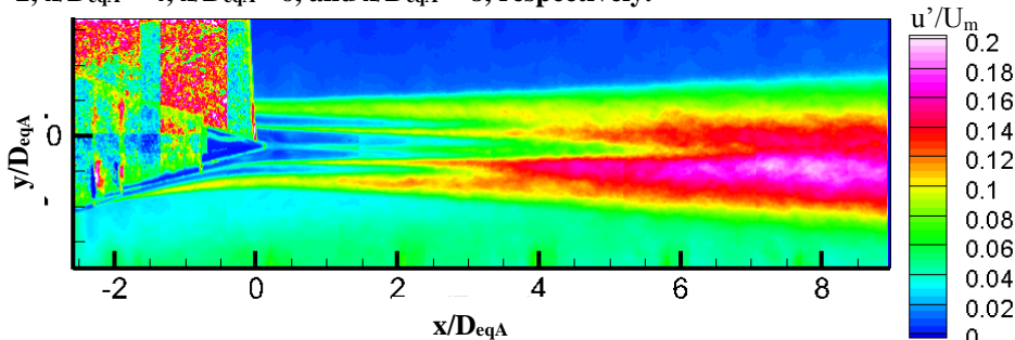
Figure 33. The turbulence intensity in the center plane for the heated three-stream jet and NPR_t = 2.1 . The data were acquired with A_b/A_c = 1 and M_{fj} = 0.3 .
