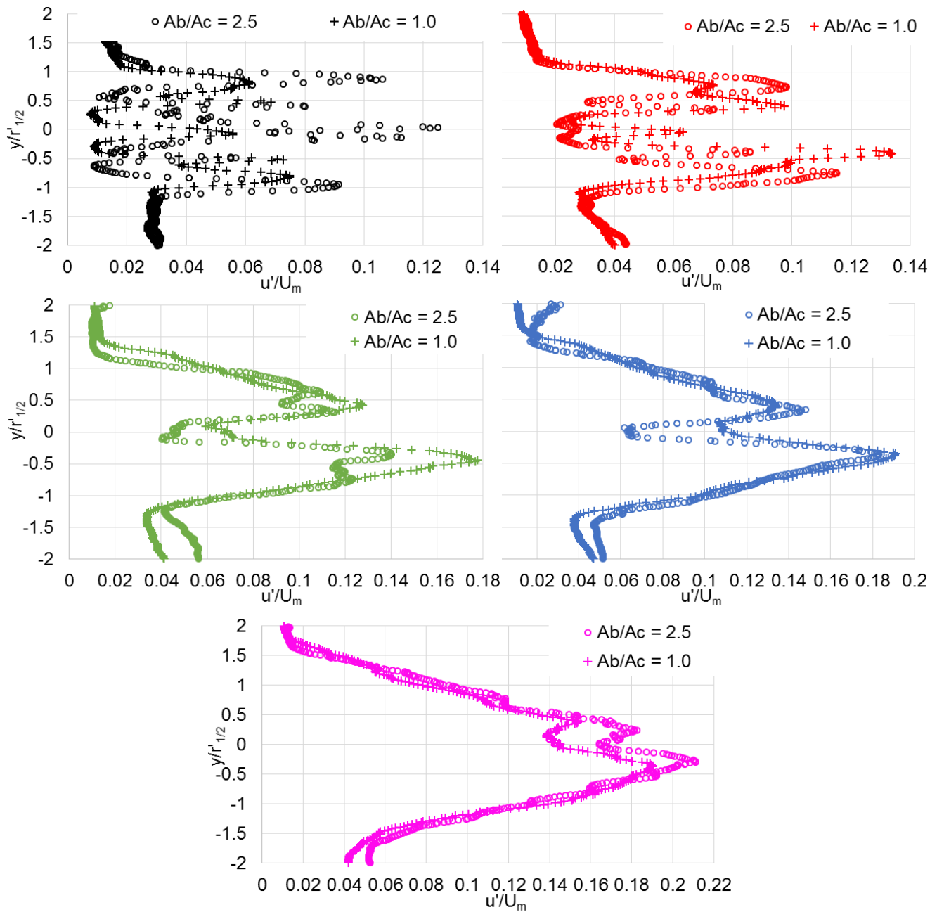
Figure 35. The turbulence intensity for the heated three-stream jets with NPR_t = 1.4 and the indicated bypass-to-core area ratio. The data were acquired with A_t/A_c = 1.0 and at M_{fj} = 0.3 . Black, red, green, blue, and magenta indicate x/D_{eqA} = 0 , x/D_{eqA} = 2 , x/D_{eqA} = 4 , x/D_{eqA} = 5 , and x/D_{eqA} = 7 , respectively.
