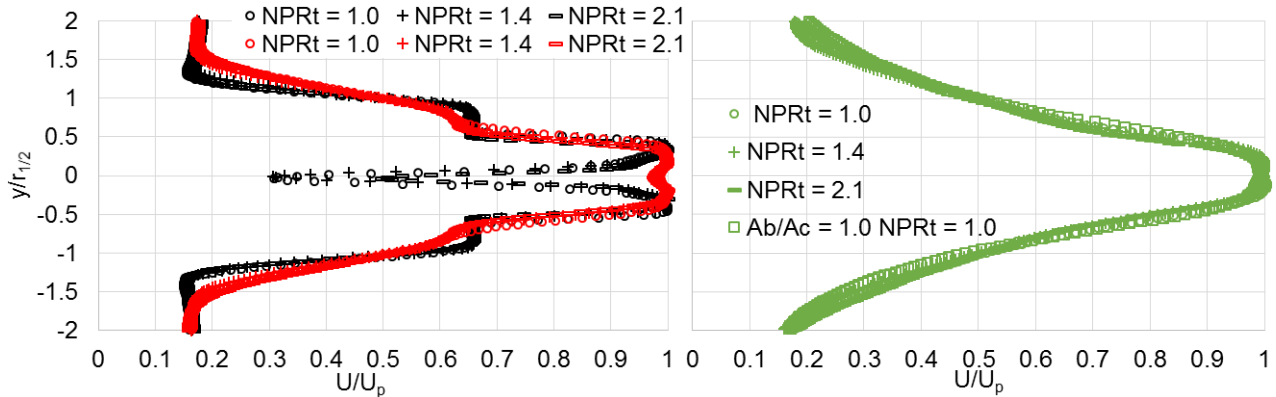
Figure 22. The velocity for the heated dual- and three-stream jets. Unless otherwise indicated, the data are for A_b/A_c = 2.5 . Black, red, and green symbols indicate x/D_{eqA} = 0, 2 and 4 , respectively. The data are for M_{fj} = 0.3 .
