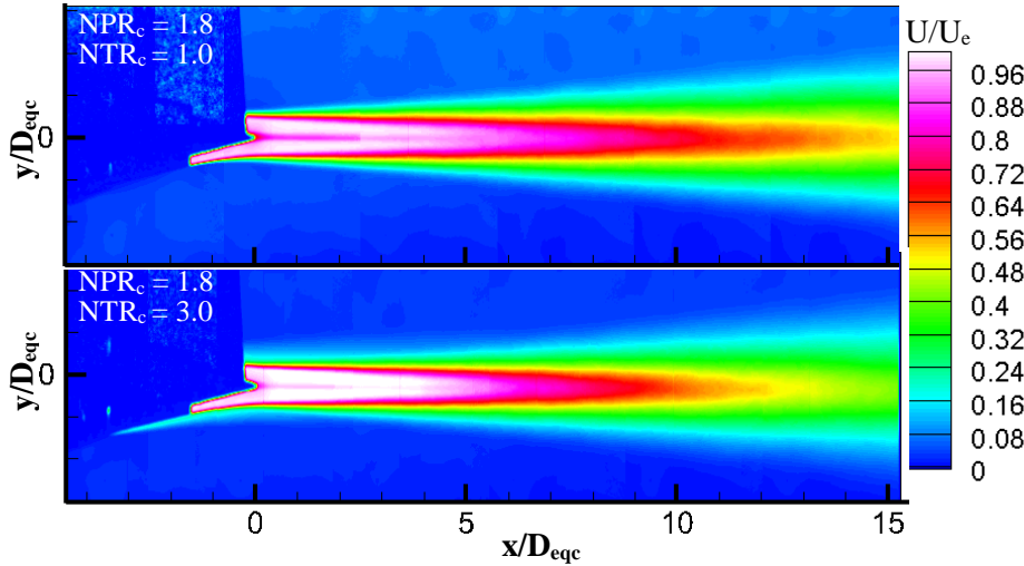
Figure 4. The velocity in the center plane for the unheated and heated single-stream jets. The data were acquired at M_{fj} = 0.0 .
