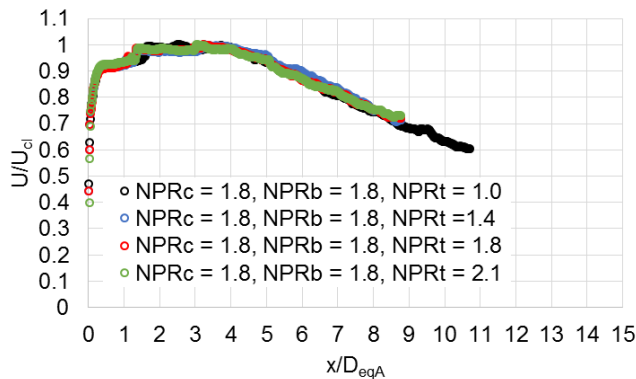
Figure 11. The centerline velocities for the indicated nozzle pressure ratios and NTR_c = 3.0 . The data were acquired for A_b/A_c = A_t/A_c = 1.0 and M_{fj} = 0.3 .
