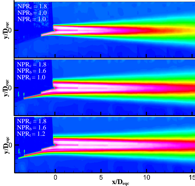
Figure 7. The velocities in the center plane for the unheated single-, dual-, and three-stream jets. The conditions are indicated on the contour plots. The legend is the same as that in Fig. 4 with U_c equal to the core exit velocity. The data were acquired for M_{fj} = 0.0 .
