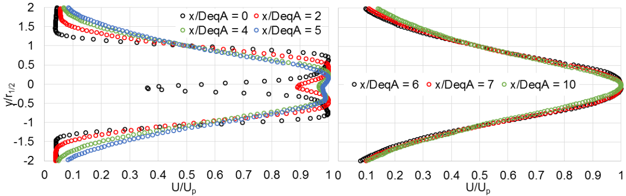
Figure 13. The velocity at the indicated cross-stream planes for the unheated single-stream jet and M_{fj} = 0.0 .
