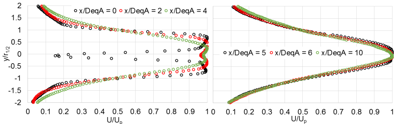
Figure 14. The velocity at the indicated cross-stream planes for the heated single-stream jet and M_{fj} = 0.0 .
