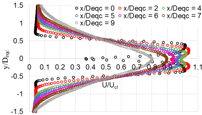
Figure 5. The velocity at the indicated cross-stream planes for the simulated single-stream unheated jet.
