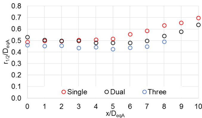
Figure 18. The half-velocity radii for the unheated single-, dual-, and three-stream jets. The data were acquired with the A_b/A_c = A_t/A_c = 1.0 and for M_{fj} = 0.0 .
