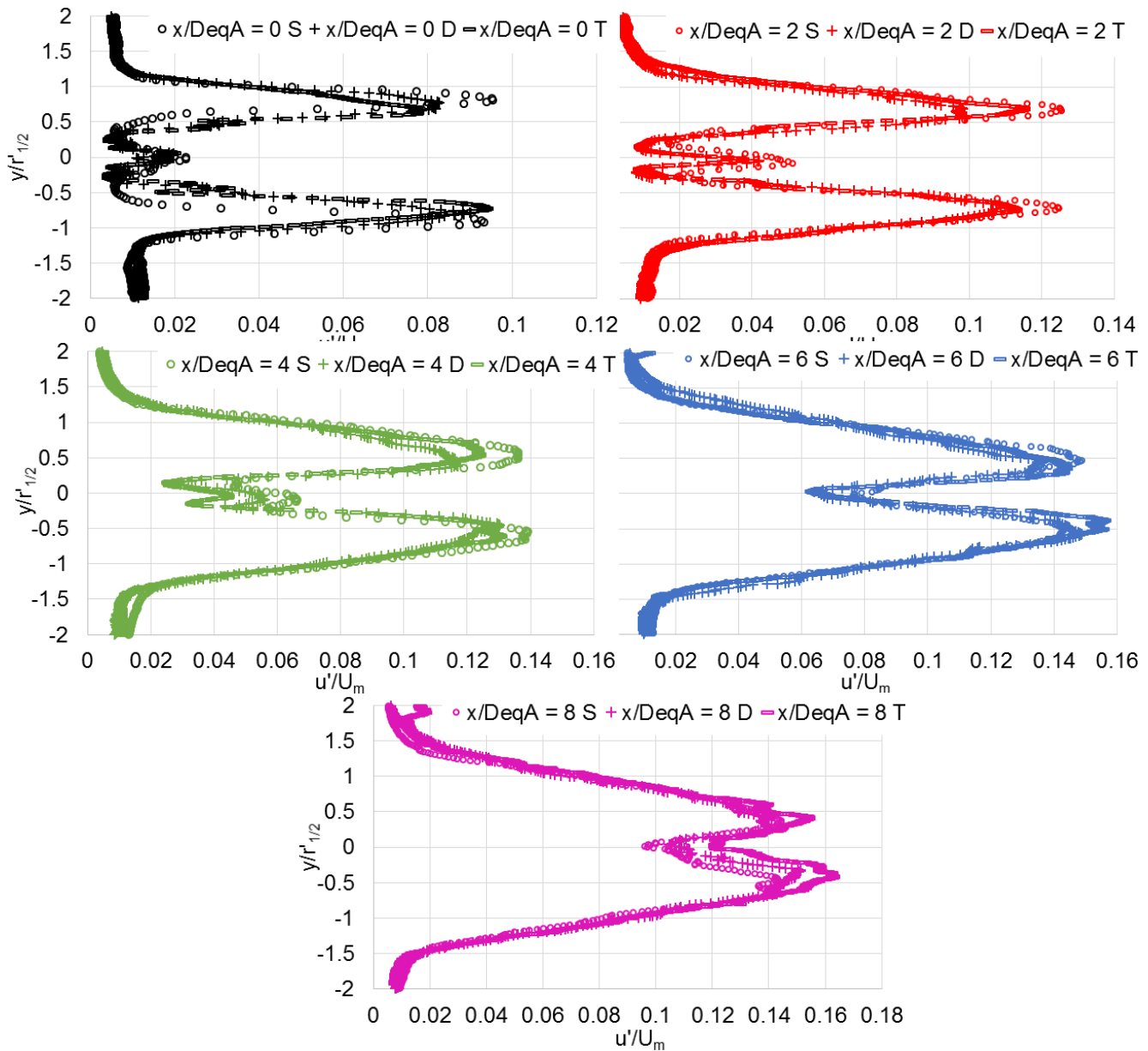
Figure 31. The turbulence intensity for the unheated single-stream (S), dual-stream (D), and three-stream (T) jets. The data were acquired with A_b/A_c = A_t/A_c = 1 and at M_{fj} = 0.0 . Black, red, green, blue, and magenta indicate x/D_{eqA} = 0, x/D_{eqA} = 2, x/D_{eqA} = 4, x/D_{eqA} = 6, x/D_{eqA} = 8 .
