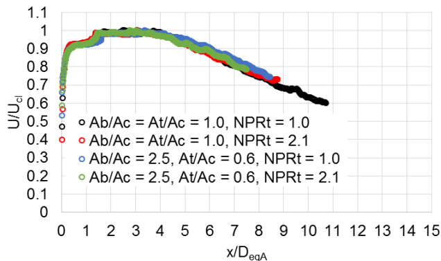
Figure 12. The centerline velocities for NPR_c = 1.8 , NPR_b = 1.8 , NTR_c = 3.0 , and the indicated area ratios and NPR_t . The data were acquired for M_{fj} = 0.3 .
