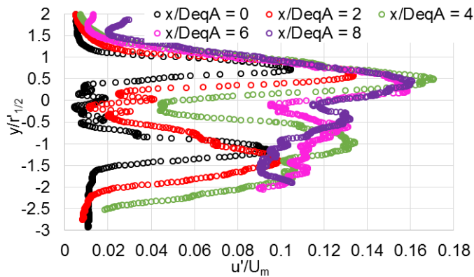
Figure 37. The turbulence intensity in the indicated cross-stream planes for the unheated offset three-stream jet with NPR_t = 1.8 and M_{fj} = 0.0 .
