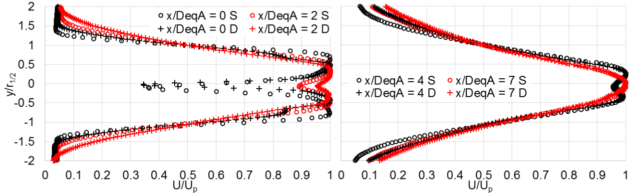
Figure 16. The velocity at the indicated cross-stream planes for the unheated single-stream (S) and dual-stream (D) jets. The data were acquired at M_{fj} = 0.0 with the A_b/A_c = 1.0 nozzle system.
