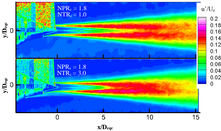
Figure 28. The turbulence intensity for the unheated (top) and heated (bottom) single-stream jets. The data were acquired at M_{fj} = 0.0 .
