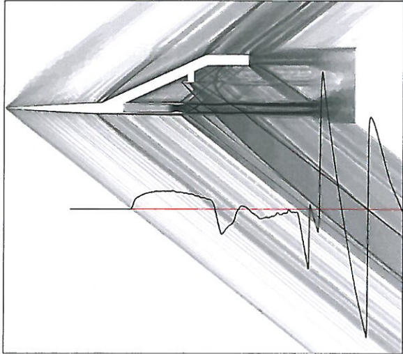
Figure 34. Density gradient of the double-wedge shock generator at 15 inches and NPR 8.
