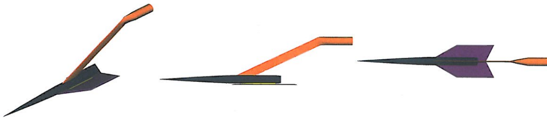
a) Isometric view b) side c) top Figure 27. Reduced size deck with nozzle exit 1.8 diameters from trailing edge.
