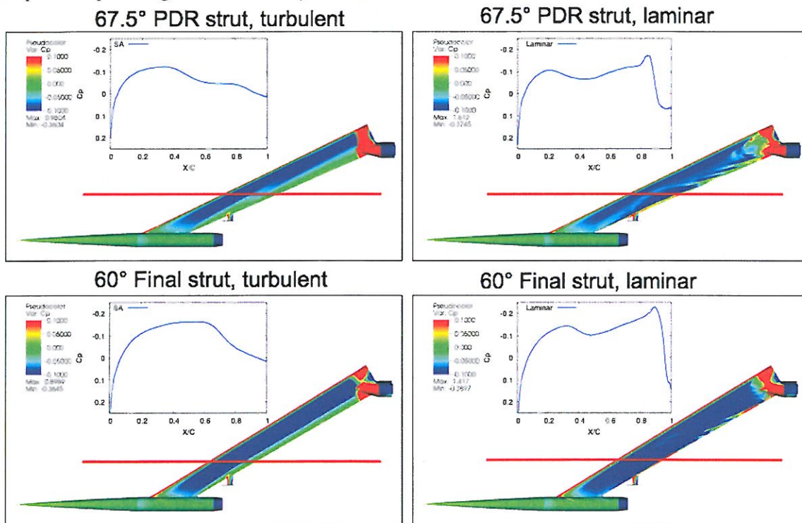
Figure 41. Pressure coefficient comparison of laminar and turbulent flow solutions for PDR and final designs.
