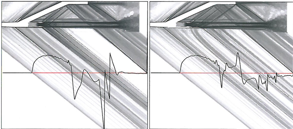
a) No deck b) Deck with nozzle exit 2 dia. from trailing edge
