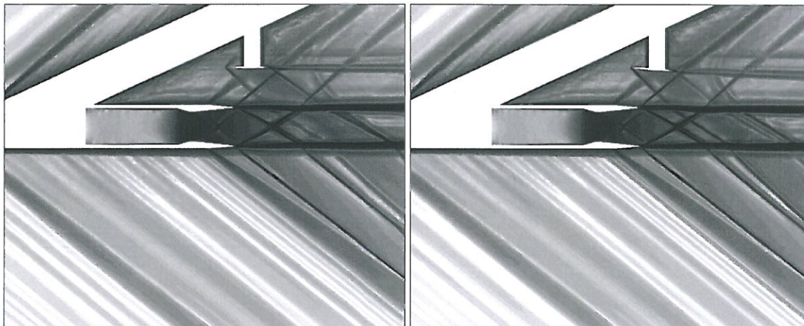
a) alpha 0^\circ b) alpha 4^\circ Figure 13. Density contours of the biconvex shock generator, M=1.6 , NPR=8 .
