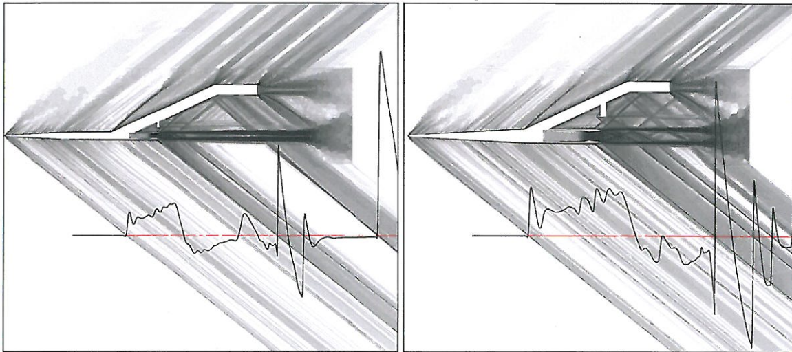
a) 1-inch diameter body and 1.0-inch biconvex SG b) 2-inch diameter body and 2.0-inch biconvex SG Figure 8. Pressure signatures at h=15 inches over contours of density gradient magnitude for different sized nozzle bodies with the LM equivalent area definitions.
