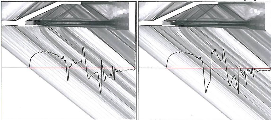
c) Deck with nozzle exit 1 dia. from trailing edge d) Deck with nozzle exit 1.8 dia. from trailing edge
