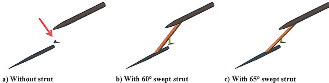
Figure 5. Isometric views of initial geometry setups with Lockheed Martin equivalent body of revolution.
