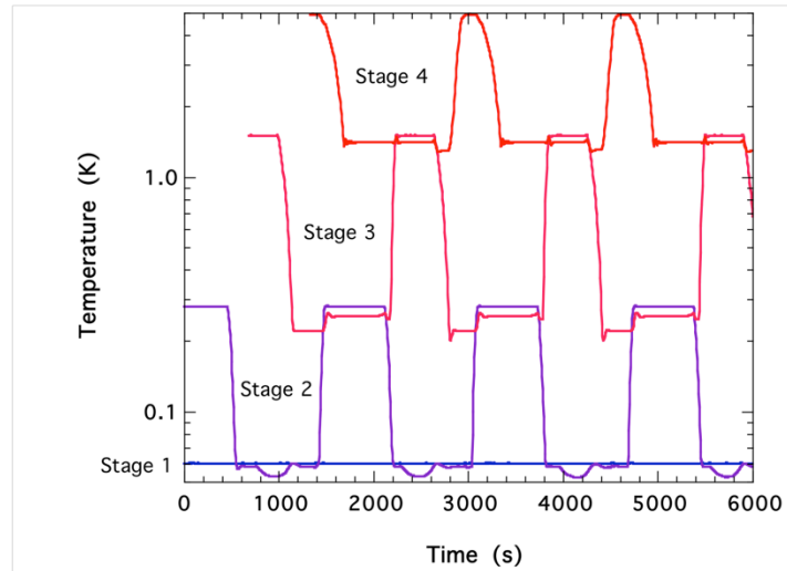
Figure 13. Cycling of a 4-stage CADR operating at 50 mK using a 4.2 K heat sink.
