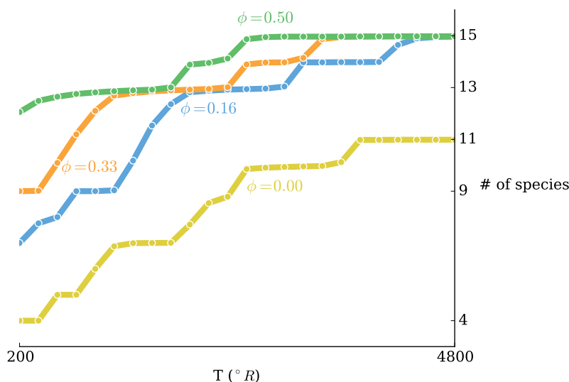
Figure 1: The total number of active chemical species in CEA equilibrium solutions over the test case set from Table 1, for a different values of \phi . The lower threshold on n_j , before a species was removed, was set to 1e-10 .
