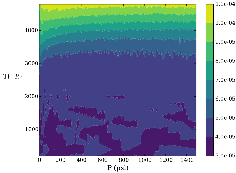
Figure 3: \|n_{\text{CEA}} - n_{\text{PyCycle}}\|_2 for \phi = .5 . This represents overall discrepancy between CEA and Pycycle at any point. There is clear trend for increasing — though still small — discrepancy as higher temperatures, and a much weaker correlation with increasing pressure.
