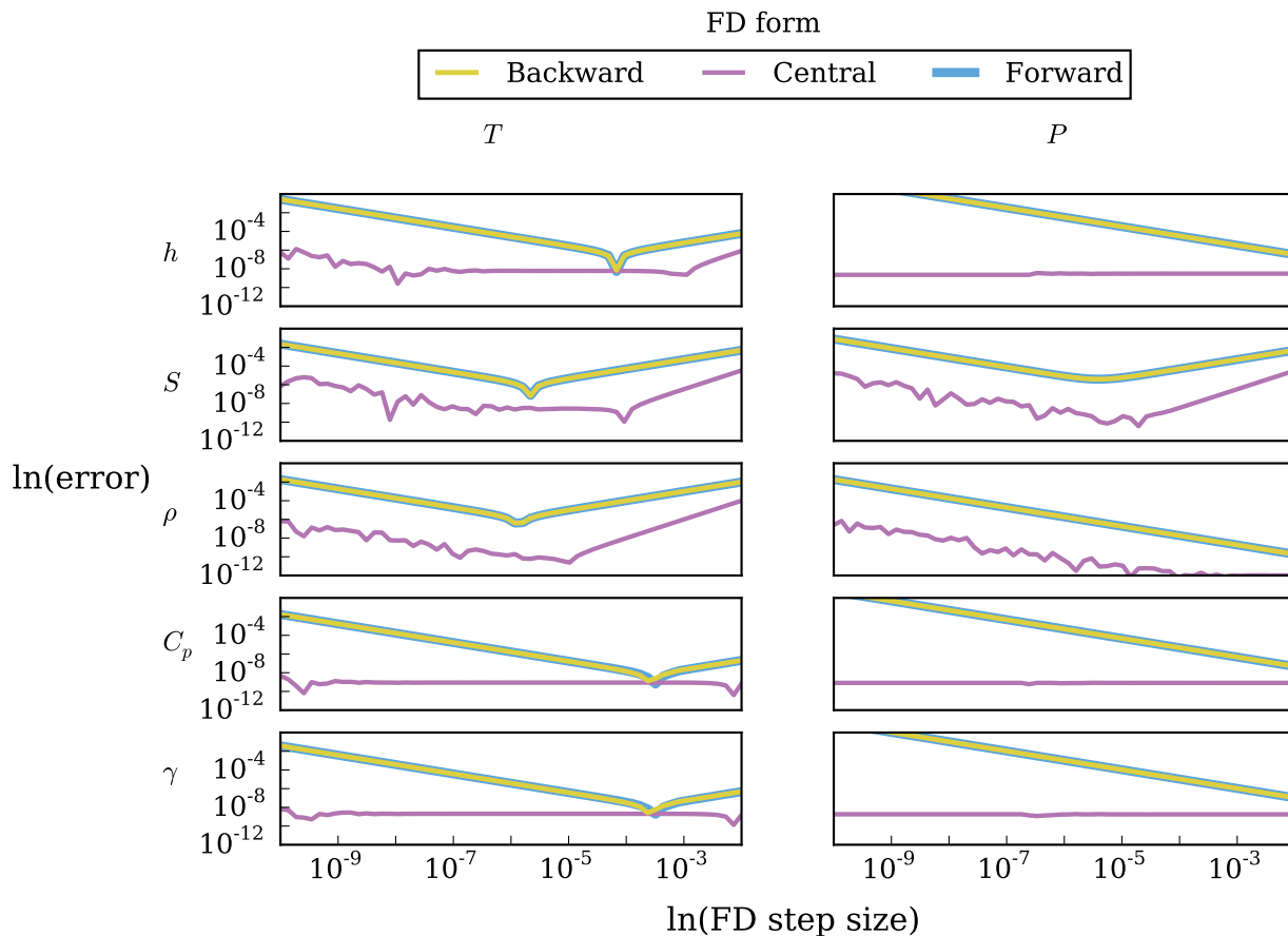
Figure 5: Finite-difference error for derivatives of h , S , \rho , C_p , \gamma with respect to T and P , taken at standard day conditions. The data is presented in a Jacobian style format, with a single row for each response and column for each independent variable. Errors below 10^{-10} were achieved at various step sizes. Notably, minimum error was found at different step sizes for different combinations of variables.
