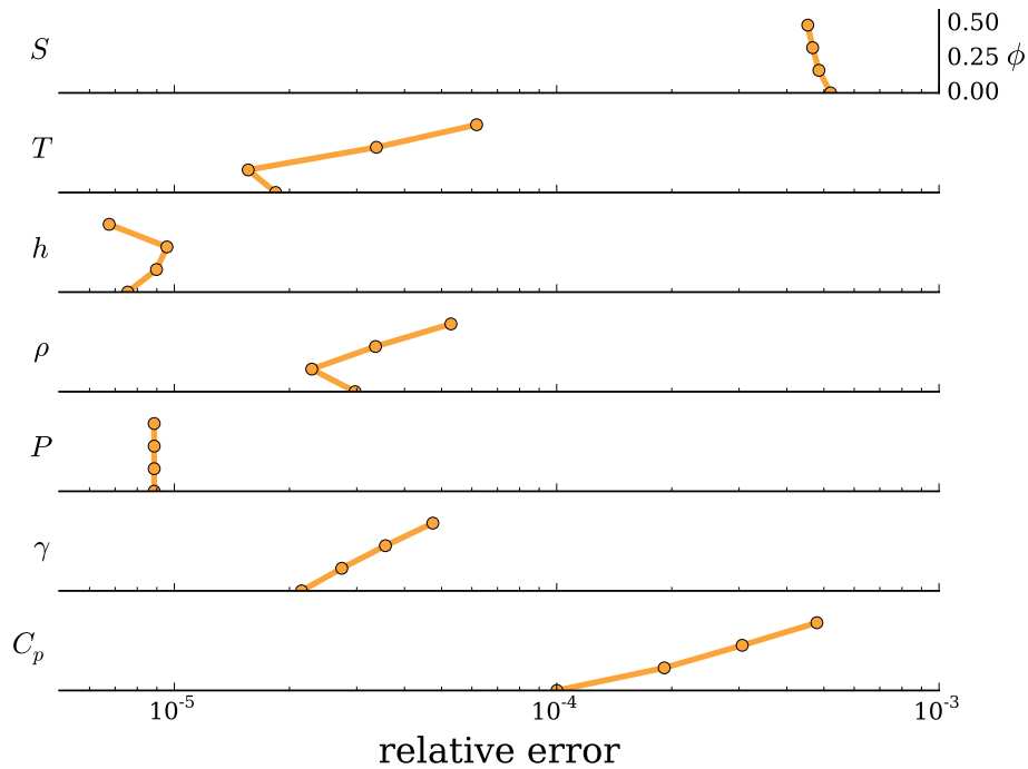
Figure 4: Mean relative error between the thermodynamics states predicted by CEA and by PyCycle sampled over the test case set from table 1.
