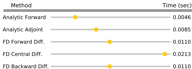
Figure 6: Wall times required to compute a full Jacobian for derivatives of h , S , \rho , C_p , \gamma with respect to T and P . All analytic methods were faster than the finite-difference methods with forward analytic being the fastest because there were 2 design variables and 5 responses. All of the compute times were generated on an Apple Macbook laptop with a 2.6 Ghz dual-core Intel Core i5 processor and 16 Gb of memory.
