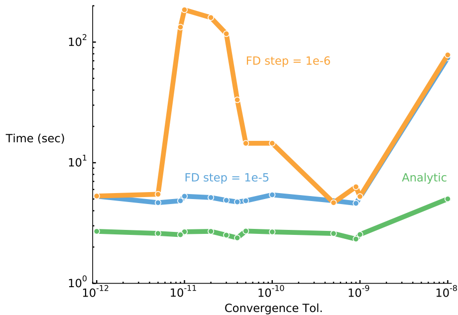
Figure 8: Optimization performance as a function of solver tolerance for the chemical equilibrium solve. The green line shows performance of the analytic derivatives method. The blue and orange lines show performance of the finite-difference derivatives for step-sizes of 1e-5 and 1e-6 respectively.
