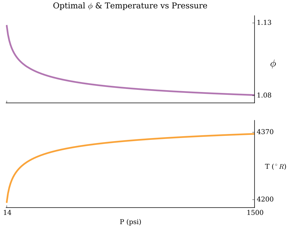
Figure 7: Optimization of Equivalence Ratio, \phi , to find maximum combustion temperature at a range of different pressures. Note that maximum temperature is reached at a slightly rich \phi due to dissociation affects, which become less pronounced at higher pressures.
