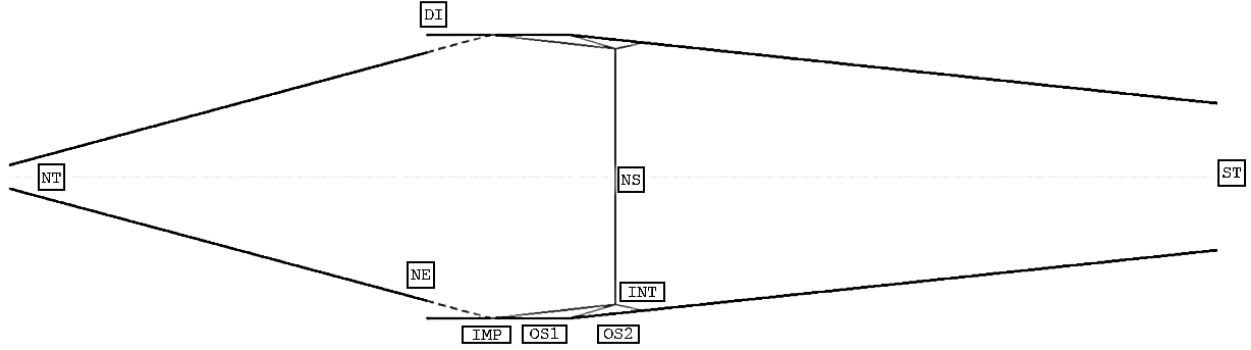
Fig. A1 - Calculation Locations for the Weighted Shocks Model
