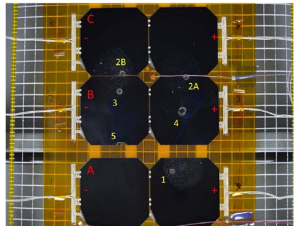
Figure 10. Impact location map for Coupon A as viewed from the front side. Nominal impact hole size is \sim 4 mm.
