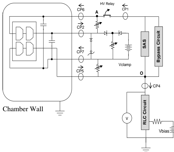
Figure 8. Electrical Schematic of Coupon A during Micrometeoroid Impact Test
