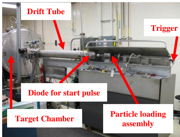
Figure 2. Side View of the Micro Light Gas Gun at the NASA MSFC Impact Test Facility
