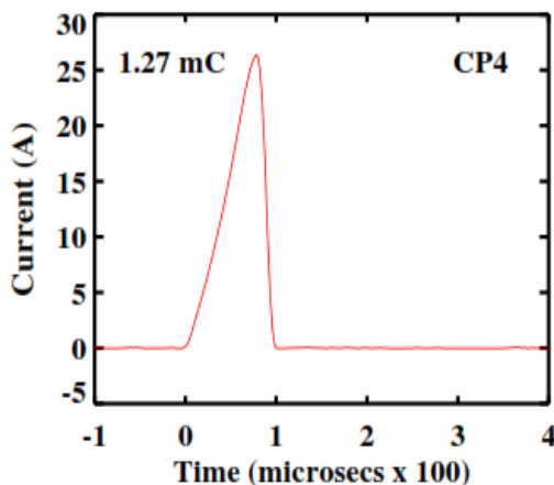
Figure 9. Primary Arc pulse used in the ESD testing. Nominal peak at \sim 25 A for \sim 100 \mu secs. Total charge contained in the pulse is \sim 1.3 mC.
