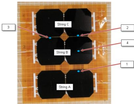
Figure 6. Coupon A Front Impact Locations
