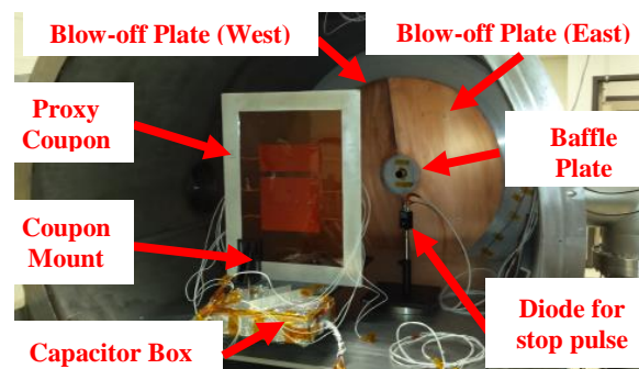
Figure 5. Target chamber layout. A mounting fixture allows adjustment of coupon for precise targeting. A laser mounted at the beginning of the drift tube aids in coupon alignment.
