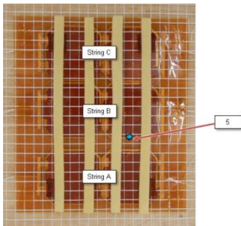
Figure 7. Coupon A Rear Impact Location
