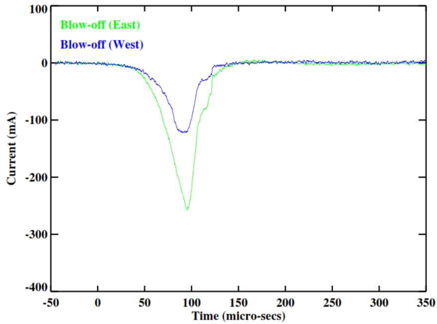
Figure 13. Blow-off plate data during impact 2B.
