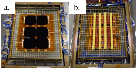
Figure 1. Micrometeoroid Test Coupon Configuration. a. front view and b. back view
