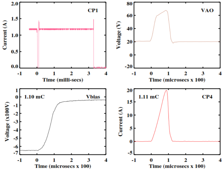
Figure 11. Current and voltage probe data for impact 2B. CP1 shows SAS current flow and is stopped by the arc interruption circuit at ~ 3 milli-sec. The charge contained in the primary arc is calculated via two methods and is noted on the Vbias and CP4 panels. A small difference in primary arc amplitude and duration is noted between the proxy coupon with copper plates and Coupon A.
