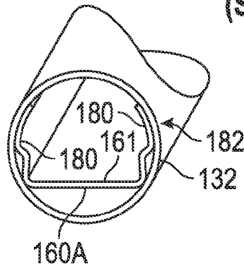
FIG. 6C (Section C-C)
