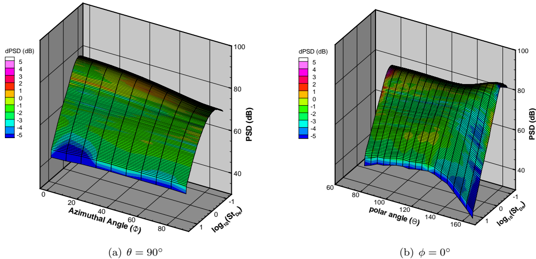
Figure 11. Predicted spectra in the azimuthal and polar arcs for setpoint 3, x_E = 4 , h_E = 0 , y_E = 2 with color contours to indicate the difference to the measured data.
