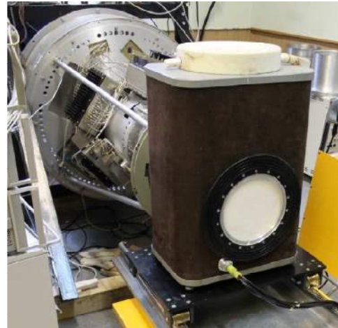
Fig. 3 Laboratory receiver calibration with load.
