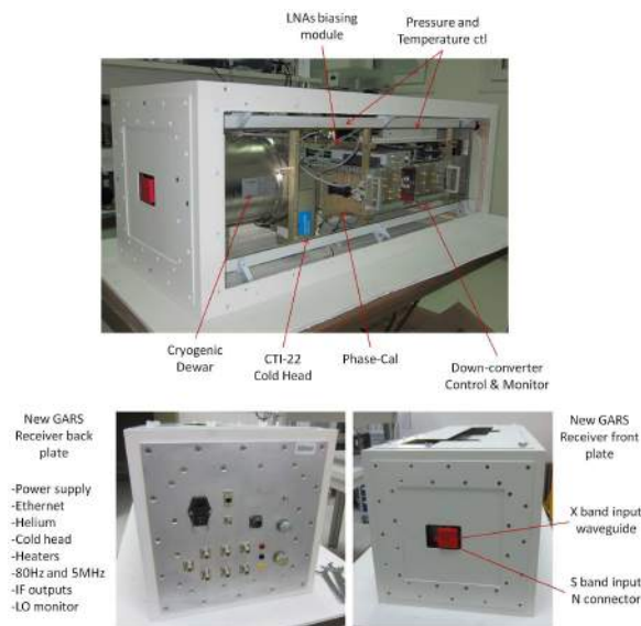
Fig. 2 The new receiver front-end at O'Higgins, which was maintained at the IVS Centro de Desarrollos Tecnológicos de Yeves, Spain.
