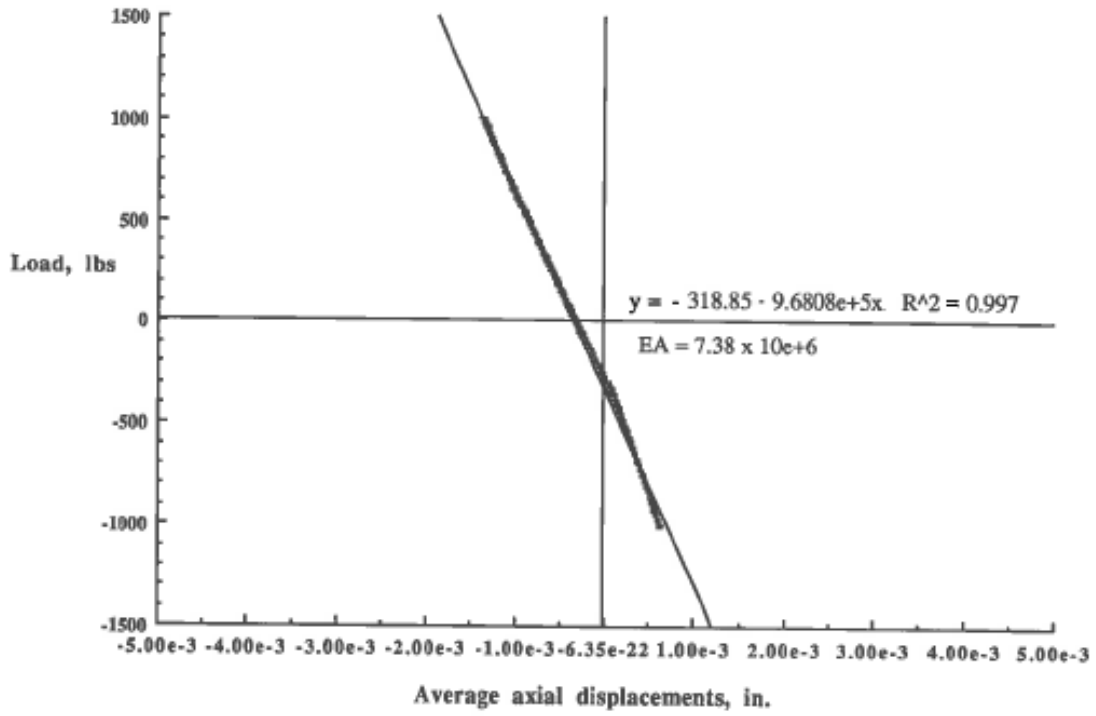
Figure A3. "Most linear" type 3 test data case.
