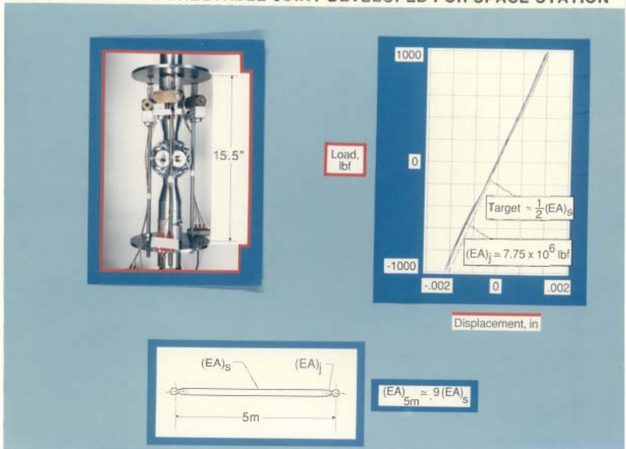
Figure A1. Type 2 Erectable joint test setup and axial stiffness data.
