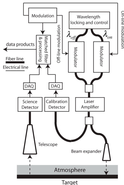
Fig. 1. Baseline instrument block diagram.
