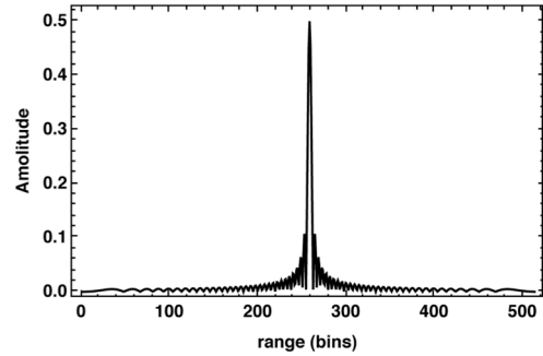
Fig. 2. Autocorrelation function using linear swept frequency modulation.
