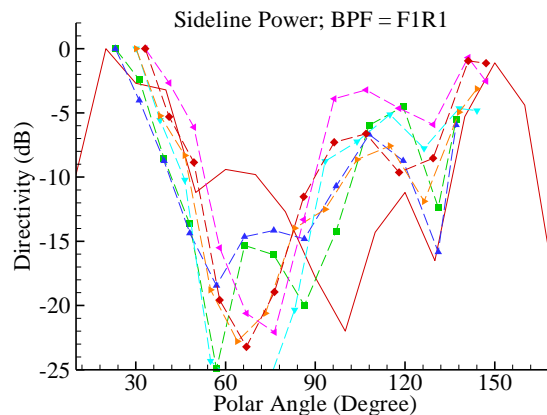
Figure 6. Directivities of the first interaction tone, F1R1, at takeoff power settings.
