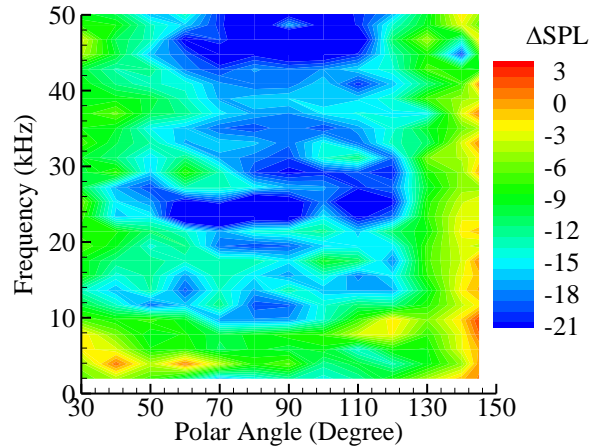
Figure 8. Shielding effects in the flyover plane for front rotor tones at takeoff power.
