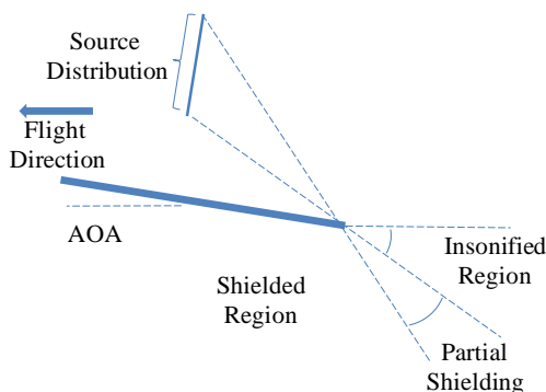
Figure 7. Illustration of general noise shielding characteristics.
