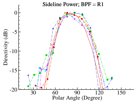
Figure 5. Directivities of aft rotor BPF, R1, at takeoff power settings.
