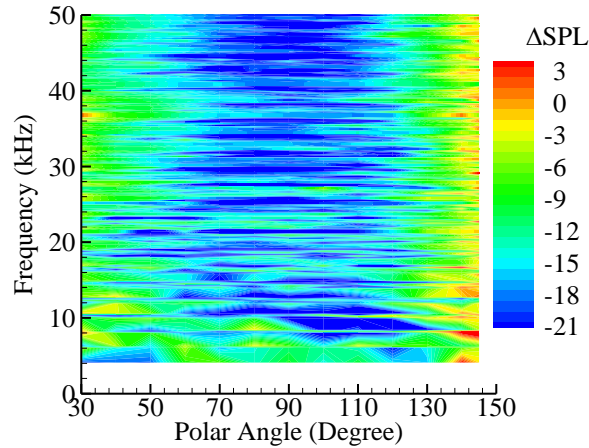
Figure 10. Shielding effects in the flyover plane for interaction tones at takeoff power.
