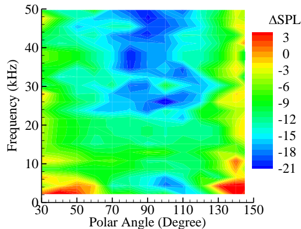
Figure 9. Shielding effects in the flyover plane for aft rotor tones at takeoff power.
