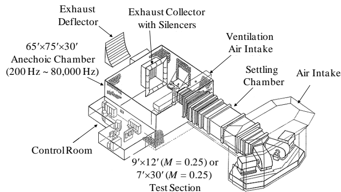
Figure 1. Boeing's Low Speed Aeroacoustic Facility (LSAF).
