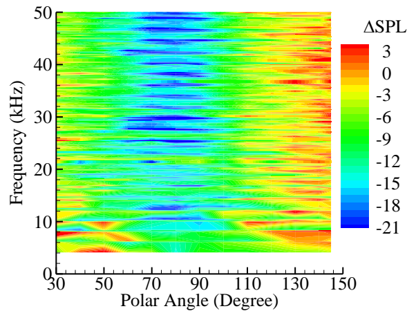
Figure 11. Shielding effects at sideline locations for interaction tones at takeoff power.
