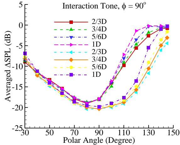
Figure 15. Shielding on interaction tones for various rotor positions in vertical direction.
