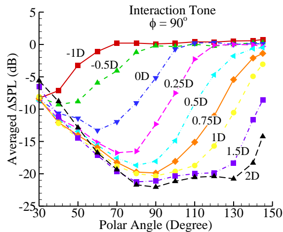
Figure 14. Shielding on interaction tones at various rotor positions in flow direction.
