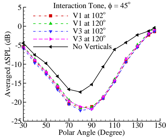
Figure 17. Effects of vertical tails on interaction tone shielding in near side direction.
