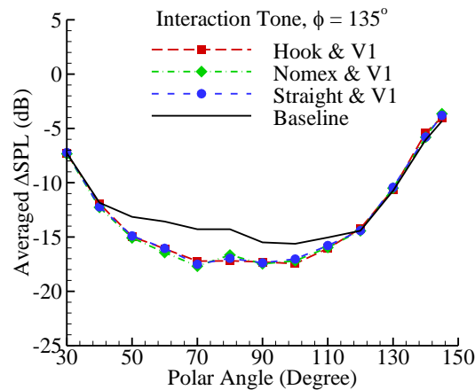
Figure 21. Effects of liner and vertical tails on far side shielding of interaction tones.
