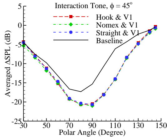
Figure 20. Effects of liner and vertical tails on near side shielding of interaction tones.
