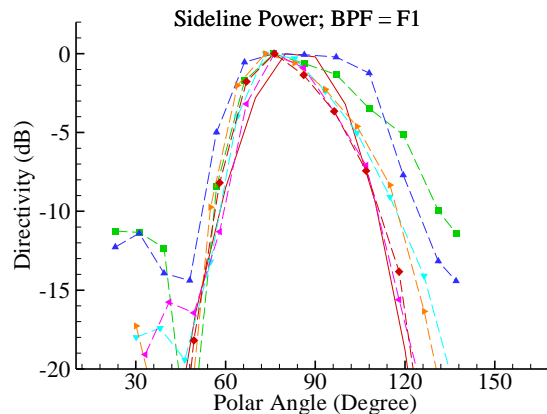
Figure 4. Directivities of front rotor BPF, F1, at takeoff power settings.
