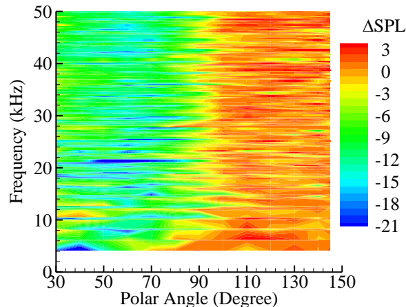
Figure 12. Shielding effects of interaction tones with rotor center at trailing edge.
