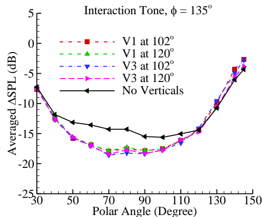
Figure 18. Effects of vertical tails on interaction tone shielding in far side direction.
