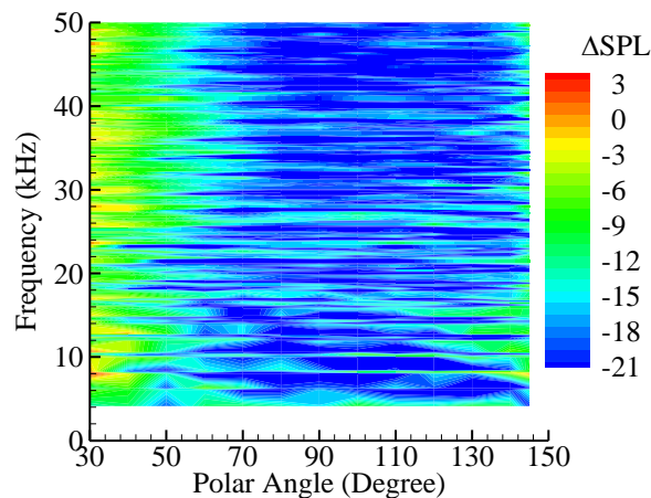
Figure 13. Shielding effects of interaction tones with rotor center 2D upstream of trailing edge.
