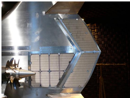
Figure 19. BWB model with local liner treatments.
