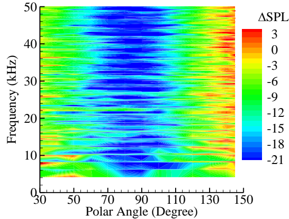
Figure 16. Shielding on interaction tones in sideline direction with V1 at 120 degrees.
