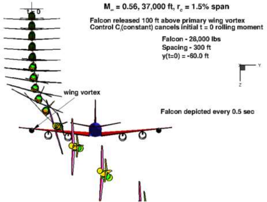
Figure 19. HU-25C Vertical Traverse, Y(0) = -60 \text{ ft} .
