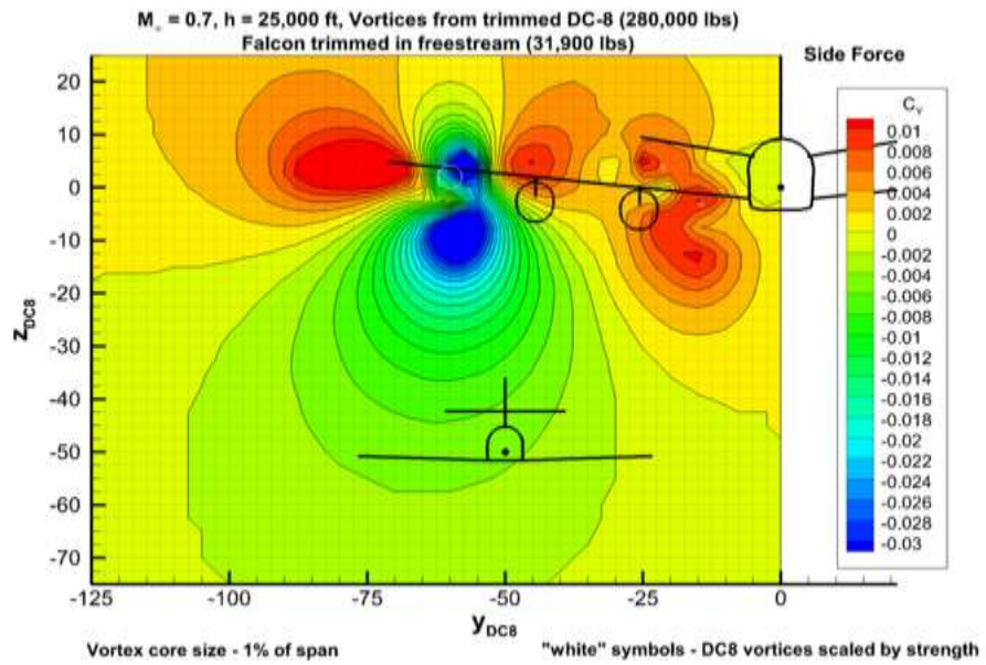
Figure 11. Induced Side Force Coefficient ( C_v ).
