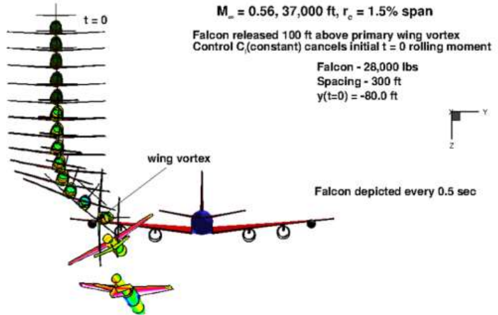
Figure 21. HU-25C Vertical Traverse, Y(0) = -80 \text{ ft} .
