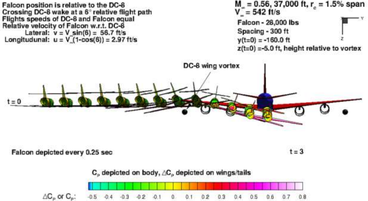
Figure 25. HU-25C Lateral Traverse, 6-Degree Heading, 5-ft. Above the Vortex.
