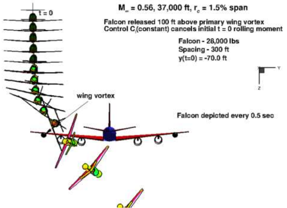
Figure 20. HU-25C Vertical Traverse, Y(0) = -70 \text{ ft} .
