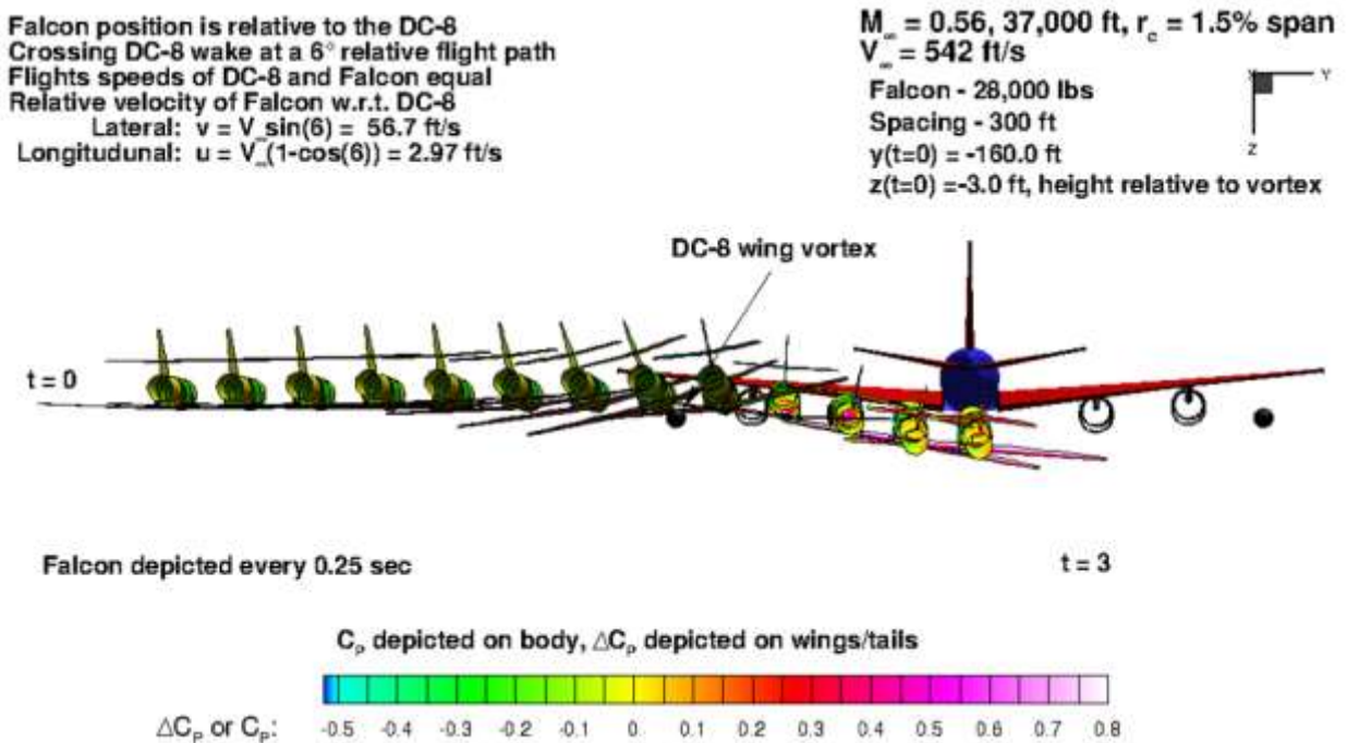
Figure 26. HU-25C Lateral Traverse, 6-Degree Heading, 3-ft. Above the Vortex.
