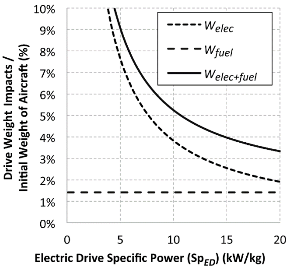
Figure 3.—Normalized weights of drive, fuel impact of inefficiency, and combined costs for 95 percent efficient drive.
