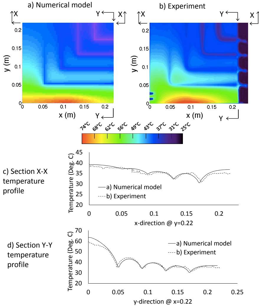
Figure 3. Numerical and experimental data correlation for: inlet pressure P_{in} = 1.2 bar and vascule inlet temperatures [T_{in}] = [T_{in,1} T_{in,2} T_{in,3} T_{in,4}] = [38 36 33 31]^{\circ}\text{C} .
