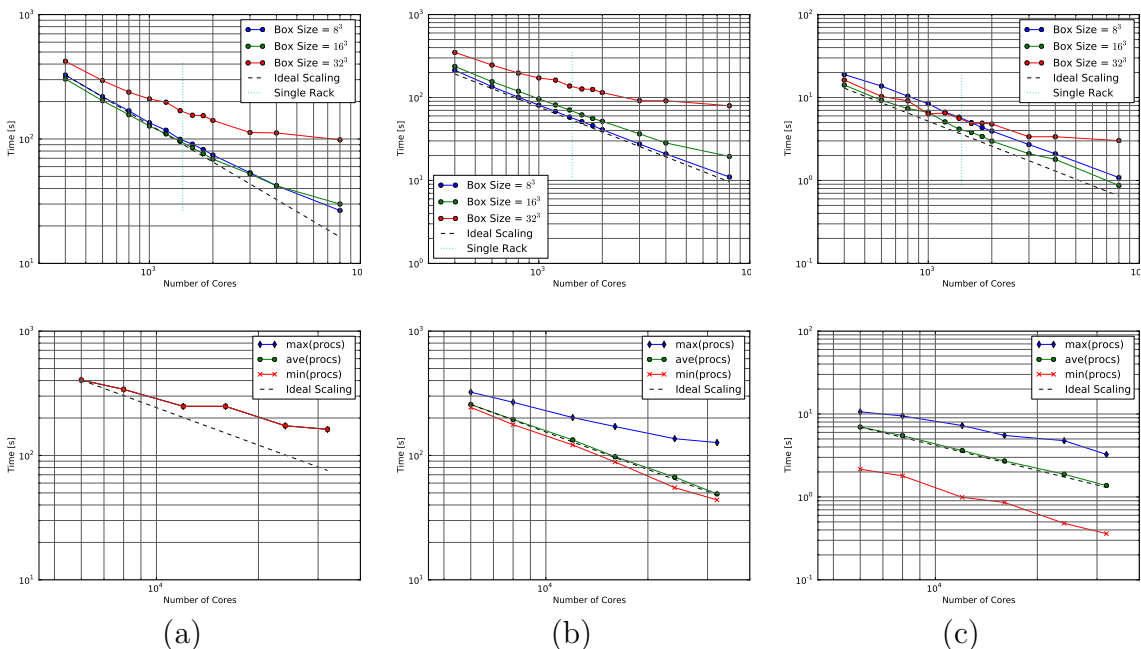
Figure 6: Strong parallel scaling study for 25 time steps: top row is \sim 300 million cells (fine mesh), max time over all procs shown; bottom row is 4.4 billion cells (super-fine mesh), min/ave/max time over all procs shown for box size of 32^3 . (a) Entire RK-solve including communication, (b) WENO-5Z flux and divergence operators, (c) immersed boundary conditions.
