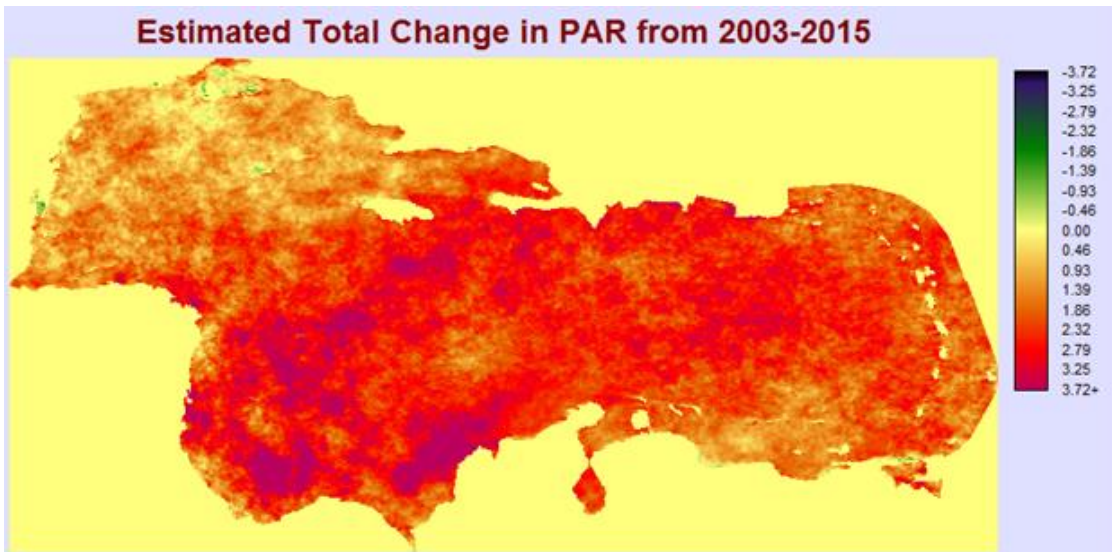
Figure 5. Total change in PAR from 2003-2015 was estimated using ordinary least squares regression. Values are in Einstein m^{-2} day^{-1} .
