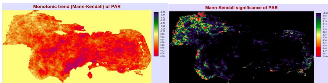
Figures 6 & 7. Results Figure 6 and significance Figure 7 (p-values) for the Mann-Kendall test applied to PAR for 2003-2015.
