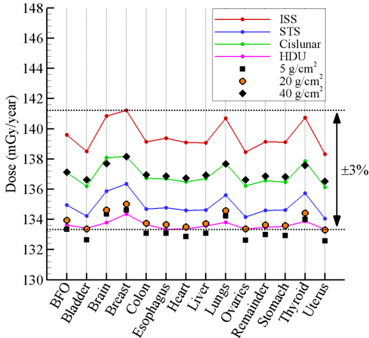
Tissue dose variation behind shielding
