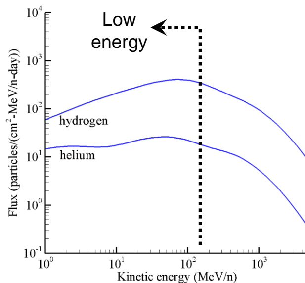
Reference field hydrogen and helium energy spectra
