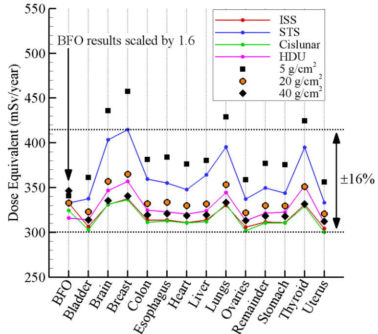
Tissue dose equivalent variation behind shielding
