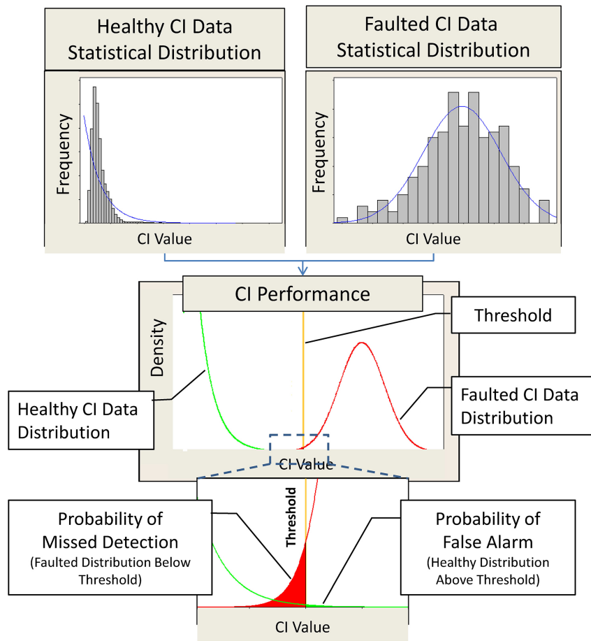
Figure 11. Analysis of Healthy and Faulted Populations to Determine CI Performance
