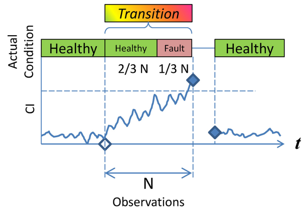
Figure 8. Final Classification of Actual Condition of Transmission
