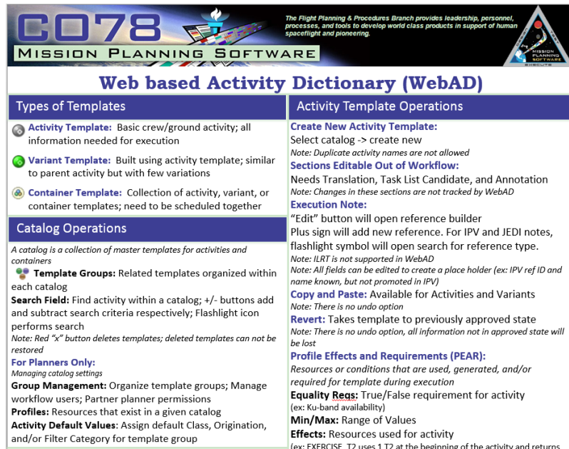
Figure 7 - Top Half of the WebAD Reference Sheet
