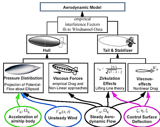
Fig. 4. Aerodynamic Model
