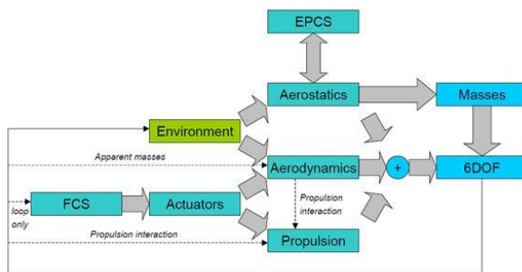
Fig. 7. Airship-Subsystem model
