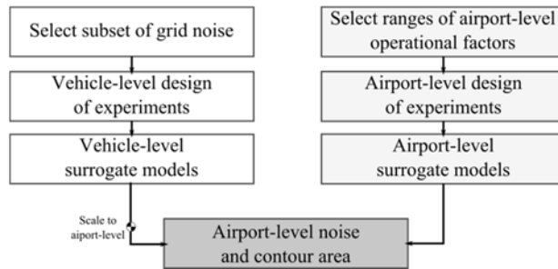
Figure 91 Approach summary. Vehicle-level and airport-level surrogates combine to predict vehicle-level impacts on the contour.
