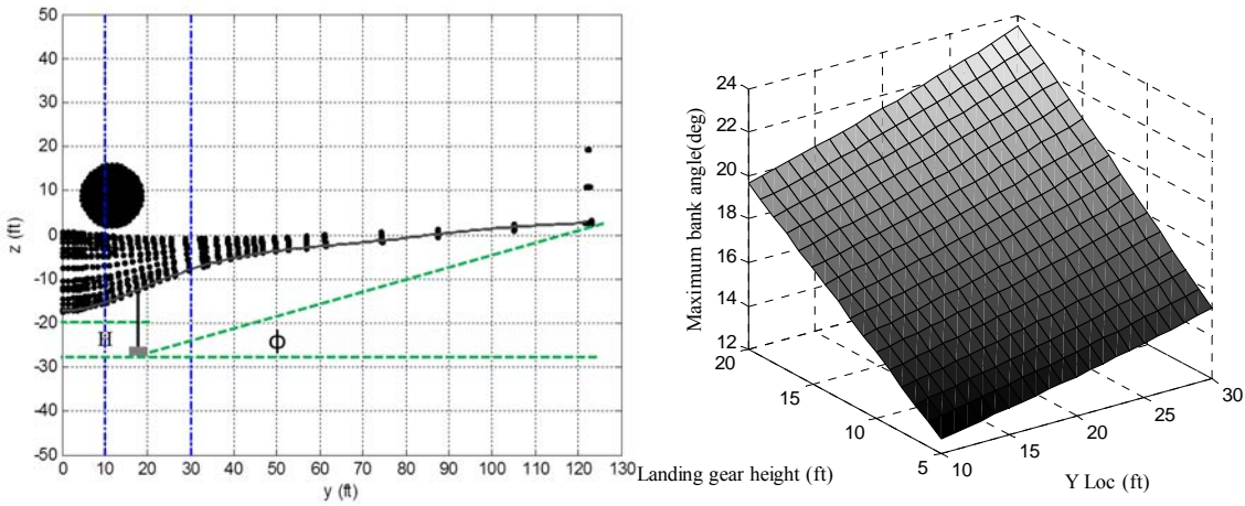
Figure 62 Wing banking clearance for the ITD HWB
