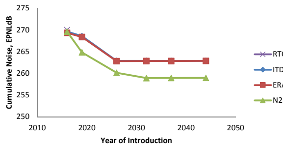
LTA - UC1 - Cumulative Noise
