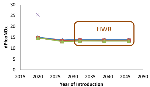
Figure 27. EDS Vehicle Emissions Performance for Fleet Scenarios - VLA Class
