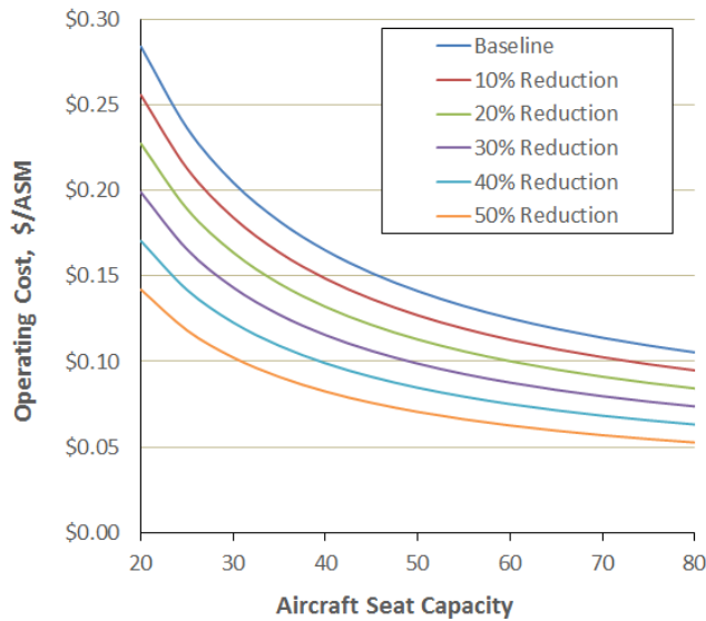
Figure 2. Operating Cost vs. Aircraft Seat Capacity.
