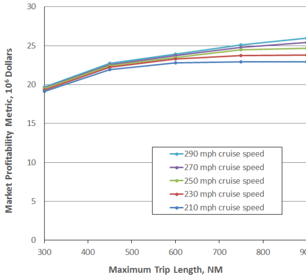
Figure 6. Sensitivity of MPM to Maximum Trip Length for Various Cruise Speeds.
