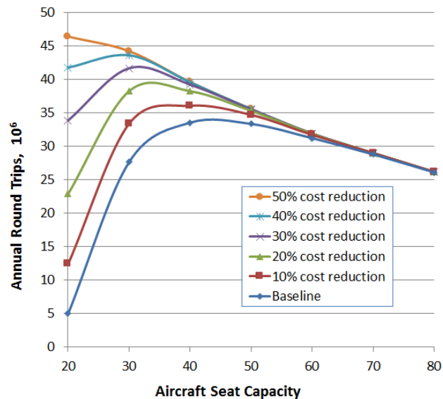
Figure 4. Number of Annual Round Trips vs. Seat Capacity for different levels of Trip Cost Reduction.
