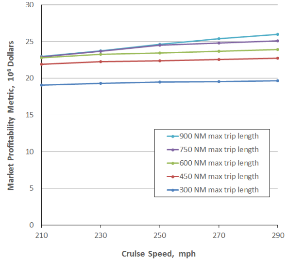
Figure 7. Sensitivity of MPM to Cruise Speed for Various Maximum Trip Lengths.
