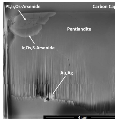
Figure 1. A bright-field STEM image of a FIB section from NWA 8186 showing a zoned arsenide and Au,Ag inclusion within pentlandite.
