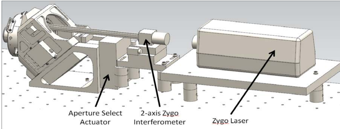
Figure 4. Interferometer Setup
