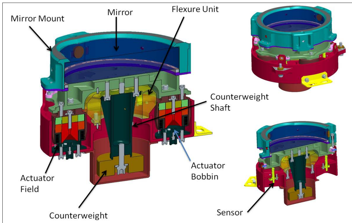
Figure 2. Cross Sections
