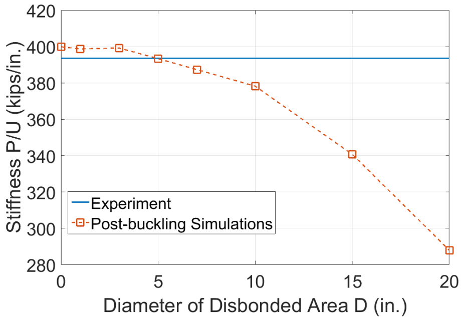
Figure 9. Stiffness evaluated at 0.1 in applied displacement \left. \frac{P}{U} \right|_{U=0.1} versus diameter D of disbonded area from FEM simulations. Stiffness from experiment on undamaged panel is also displayed for comparison.
