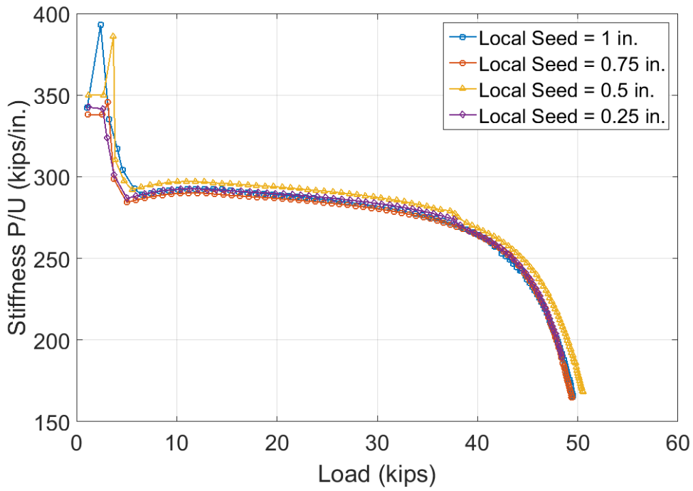
Figure 25. Sensitivity of panel stiffness ( P/U ) versus applied load to local mesh refinement in the disbanded area for a panel with a disbond of diameter D = 20 in.
