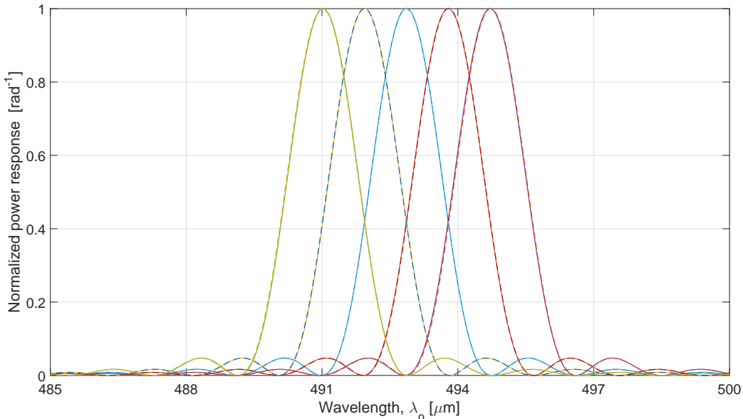
Figure 6. The angular power response for the R = 256 design. The emitter arrays angular power response (solid lines) is normalized by the total radiated power and plotted for five adjacent channels only (the full sampling of the design extends across the full wavelength band but is not shown in this plot). The dashed lines represent the ideal \text{sinc}^2 functions. One sees that the array response closely approximates this ideal function out to \sim 10 wavelengths. This \text{sinc} function remains an approximation as the emitter array antennas are not uniformly illuminated.
