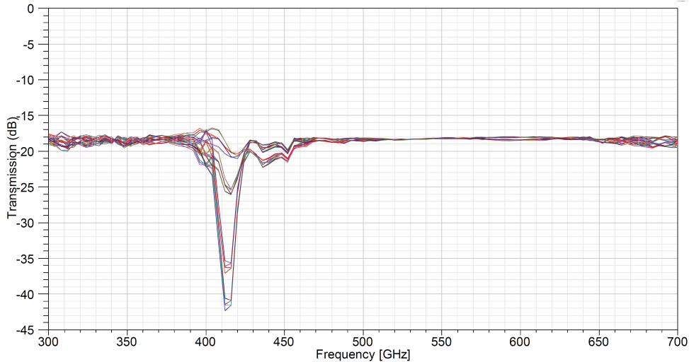
Simulated transmission from input to port N
