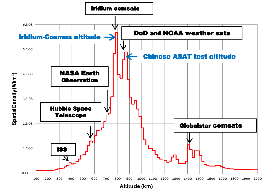
Current Estimated Density of debris at various orbital altitudes with notation of recent collisions and resulting spikes (Figure courtesy of Orbital Debris Program Office: J. C. Lui)
