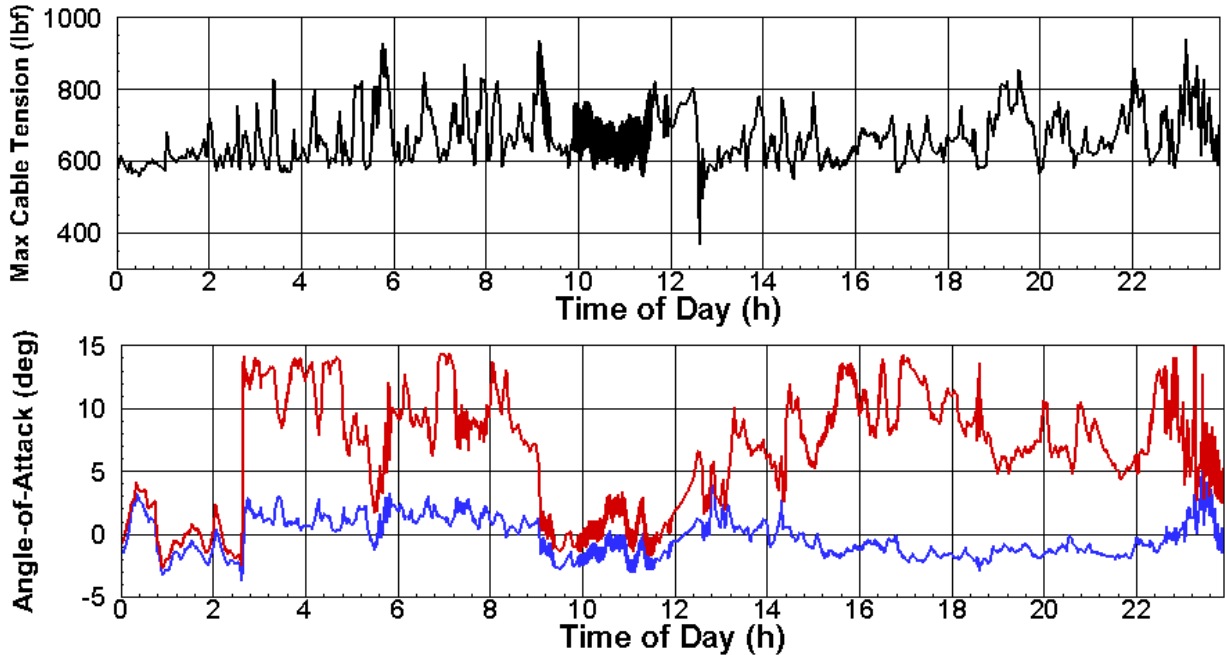
Figure 14. Trajectory histories for maximum cable tension and aircraft angle-of-attack during day #36
