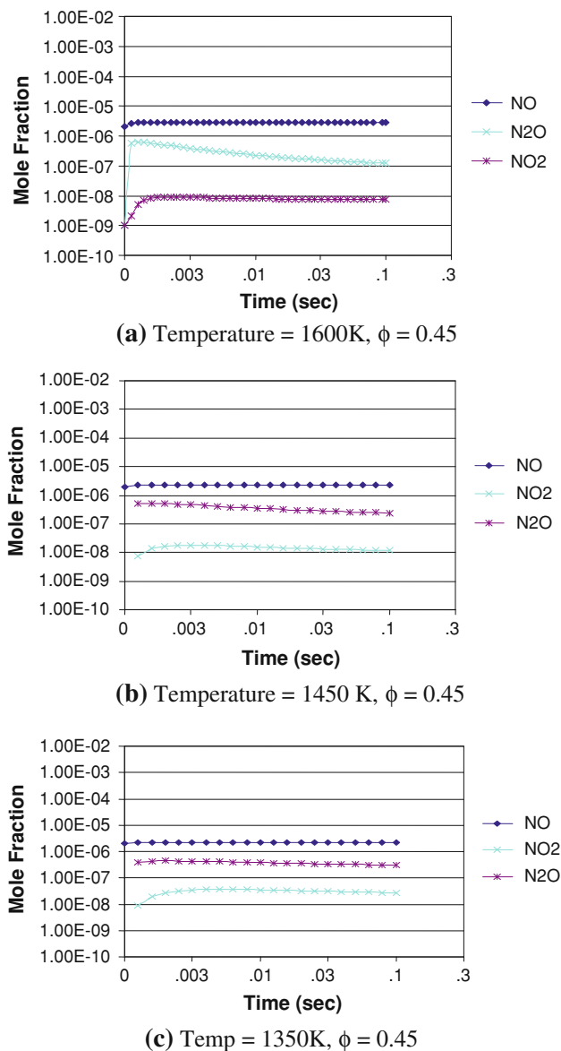
Fig. 12 Chemical kinetic evolution of primary fixed nitrogen species for \phi = 0.45 . Conditions similar to conditions in the fuel-lean zone
