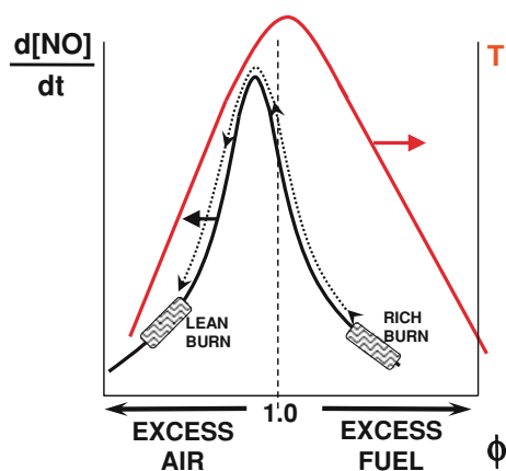
Fig. 2 RQL strategy
