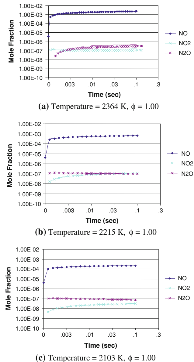
Fig. 11 Chemical kinetic evolution of primary fixed nitrogen species for \phi = 1.00
