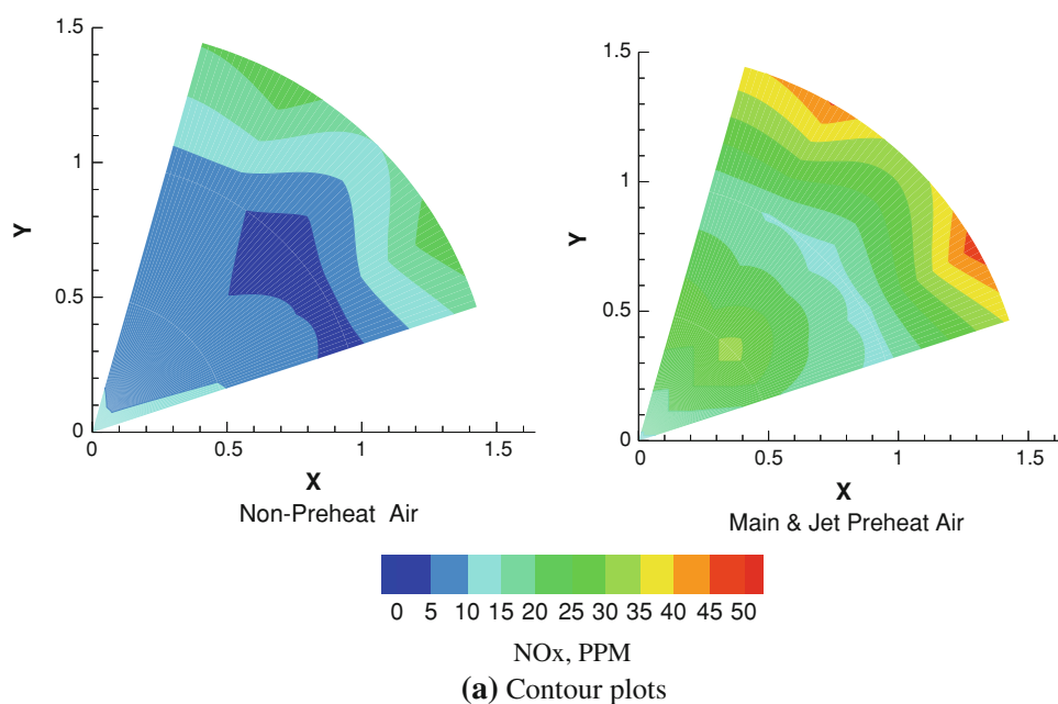
Fig. 13 Experimental \text{NO}_x data at x/R = 1 and J = 57 for the 12 hole module for non-preheat and jet and main air preheat conditions
