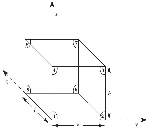
Figure 10. A typical brick element.
