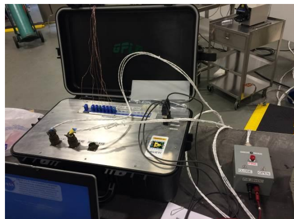
Figure 9: DAQ-in-a-Box
