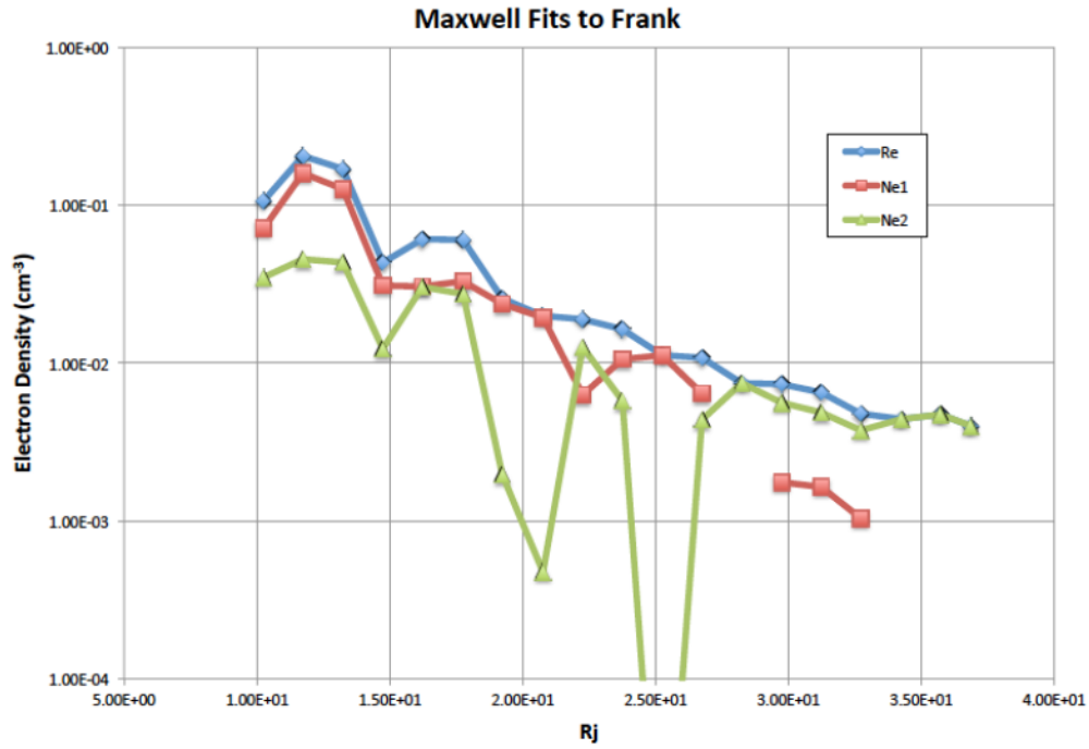
Figure 17. Fits to the E4 PLS averages from the PDS. Values plotted are the electron total density ( \text{cm}^{-3} ), low energy electron density ( \text{Ne1} , \text{cm}^{-3} ), and high energy electron density ( \text{Ne2} , \text{cm}^{-3} ).
