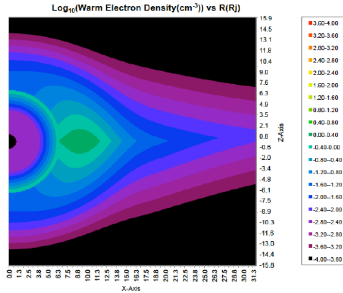
Figure A-1. Meridional contour plot of Log 10 of warm electron density at 110° W longitude.
