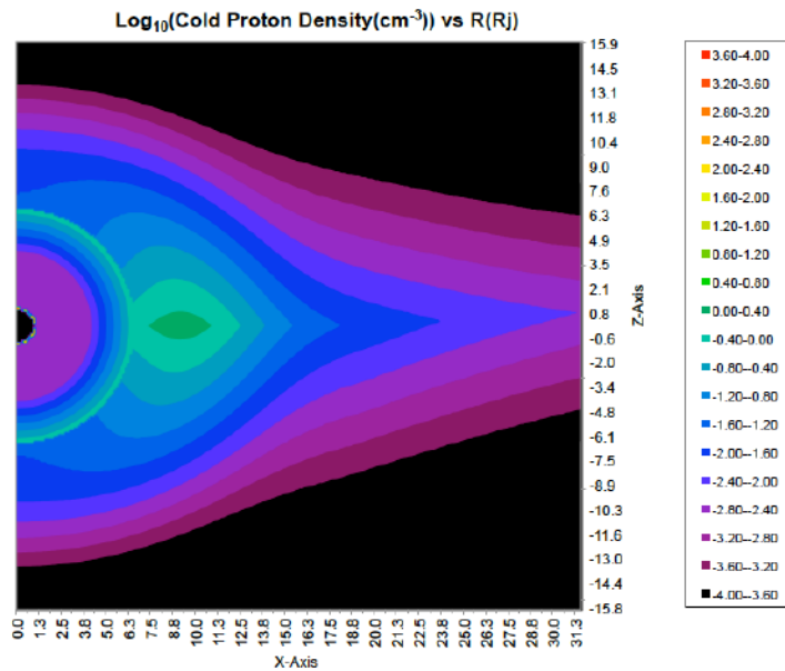
Figure A-2. Meridional contour plot of Log 10 of cold proton density at 110° W longitude. See 3.2.4 for discussion of concerns with this parameter.
