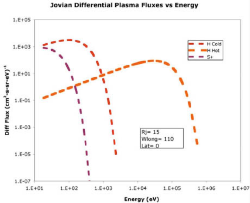
Figure 5. Background plasma differential fluxes at the base of the auroral zone at 15 Rj, 110° W, and 0° latitude (Garrett et al., 2008). Flux components are: a) cold (E Cold), warm (DFE2), high energy (DFE3), Kappa (DFE4) electrons, and Energetic Particle Detector (EPD); b) cold protons (H Cold), warm protons (H Hot), and singly ionized sulfur (DFS+)—latter assumed representative of the other cold ion species.
