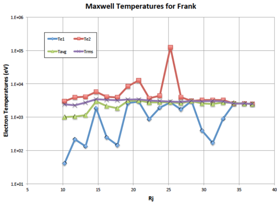
Figure 18. Fits to the E4 PLS averages from the PDS. Values plotted are the “average” electron temperature (eV), “RMS” electron temperature (eV), the low energy electron temperature component ( \text{Te1} , eV), and high energy electron temperature component ( \text{Te2} , eV).
