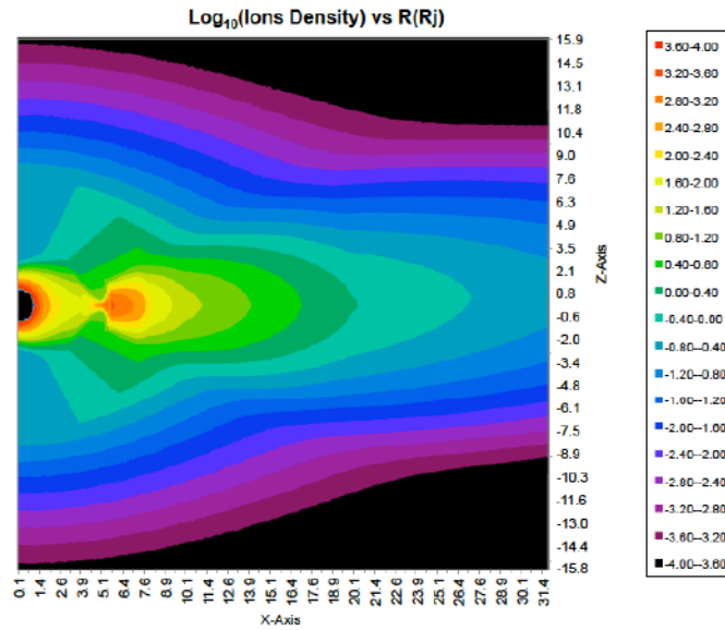
Figure A-4. Meridional contour plot of Log 10 of the total ion density plus the cold protons at 110° W longitude. See text for discussion of concerns with this parameter.
