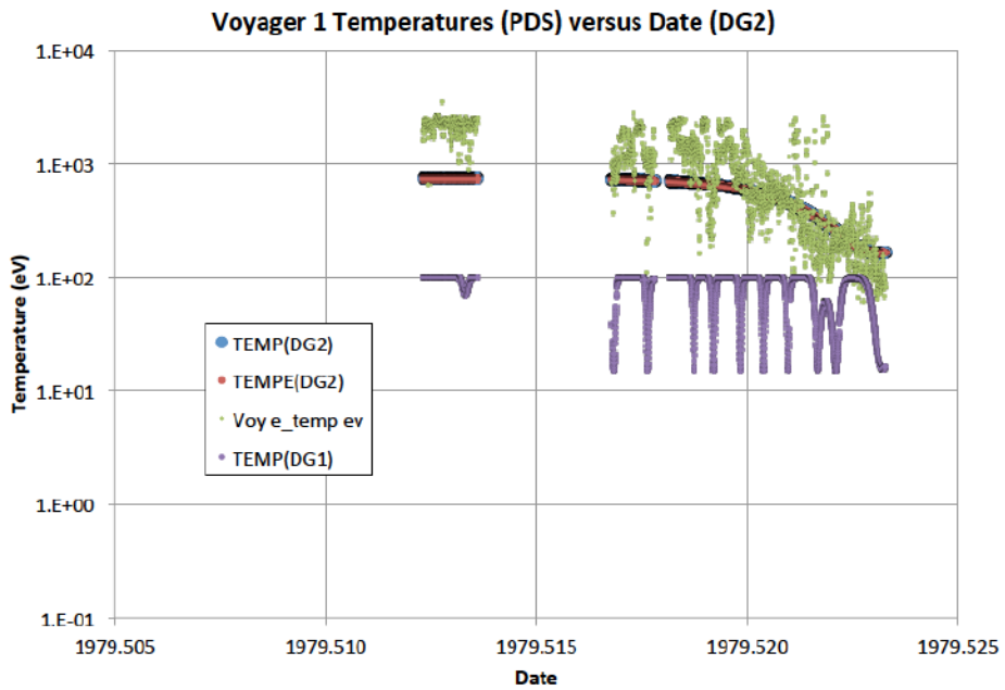
Figure 28. Voyager 1 and 2 electron temperatures versus time compared with DG1 and DG2 electron and ion temperature predictions during the Voyager flybys of Jupiter. The Voyager data (Voy e) are from the PDS (Sittler and Strobel, 1987). “TEMP(DG1)” are the cold ion and electron temperatures for the DG1 model. “TEMP(DG2)” and “TEMPE” are the cold ion and electron temperatures respectively for the DG2 model.
