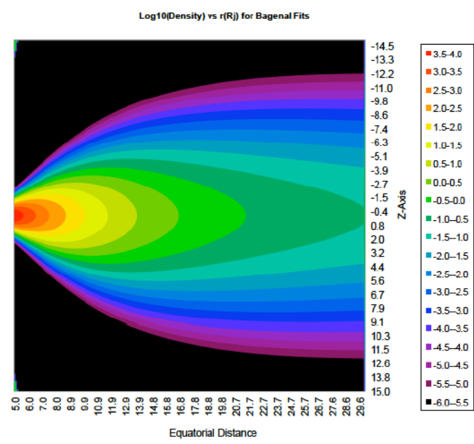
Figure 32. Log 10 of the Cold Ion Density (cm -3 ) versus R(R j ) at 110° W Longitude. Top contour is for the sum of the DG2 ions (excluding the protons) while the bottom contour is for an average contour suggested by the Bagenal and Delamere (2011) parameters. Note difference in scales.
