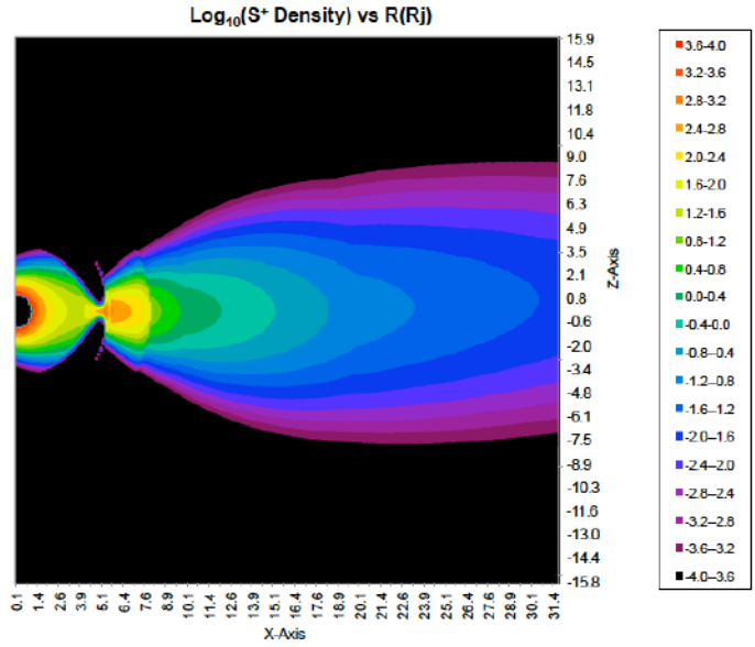
Figure A-5. Meridional contour plot of Log 10 of cold ion S + at 110° W longitude.
