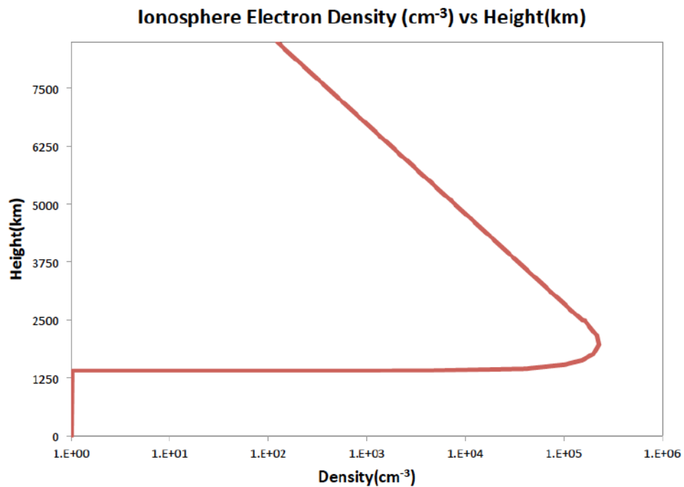
Fig. B-1. Representative jovian electron ionospheric density ( \text{cm}^{-3} ) profile between 0 km and 8500 km based on profiles from Yelle and Miller (2004). The cold ion profile is assumed to be the same.
