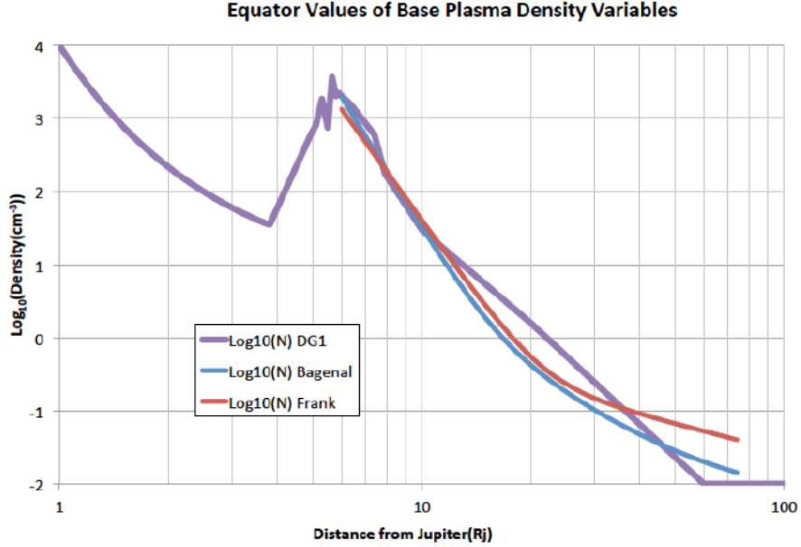
Figure 23. Plots of the ion densities versus Rj for the DG1/DG2, Bagenal, and Frank fits. The Bagenal and Frank fits are defined in Bagenal and Delamer (2011).
