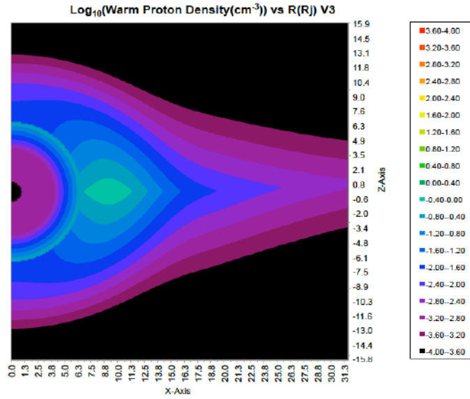
Figure A-3. Meridional contour plot of Log 10 of warm proton density at 110° W longitude.
