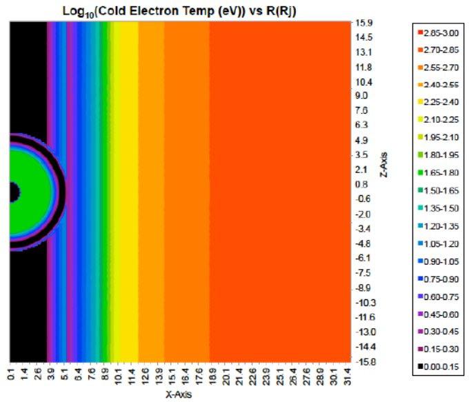
Figure A-6. Meridional contour plot of Log 10 of the cold electron temperature at 110° W longitude.
