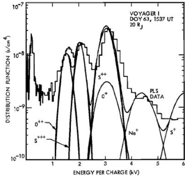
Figure 4. Comparisons for Voyager 1 Plasma Science (PLS) instrument spectra at a) 1016 UT, Day 64, at 5.3 R J and b) 1537 UT, Day 63, at 20 R J (Divine and Garrett, 1983).
