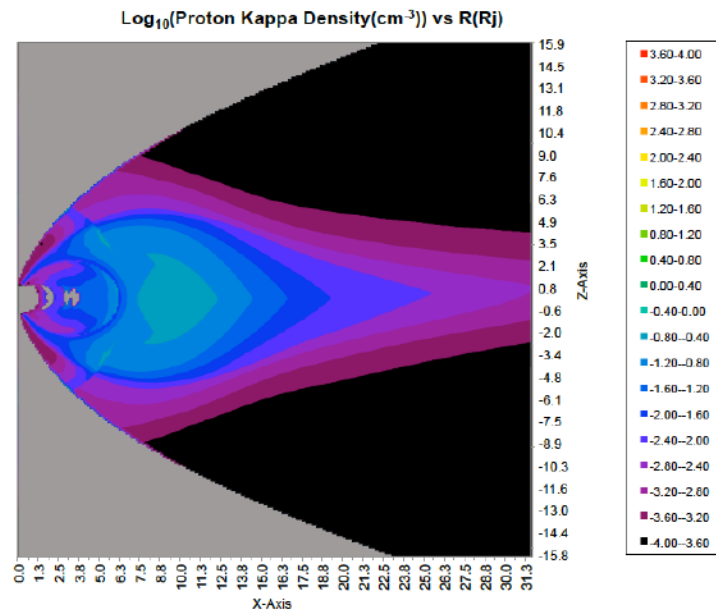
Figure 35. Meridional contour plots of the three proton Kappa plasma distribution parameters (Kappa value, density, and temperature) as modeled by the DG2 plasma model. The gray contours correspond to regions where the program could not fit a Kappa distribution—typically this was where there is no high energy proton data (e.g., outside ~60 L).
