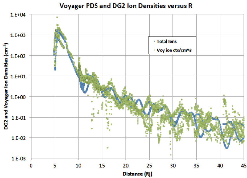
Figure 29. Voyager PDS cold electron and ion data (green dots) and DG2 predictions (blue dots) versus distance from Jupiter ( R_j ).
