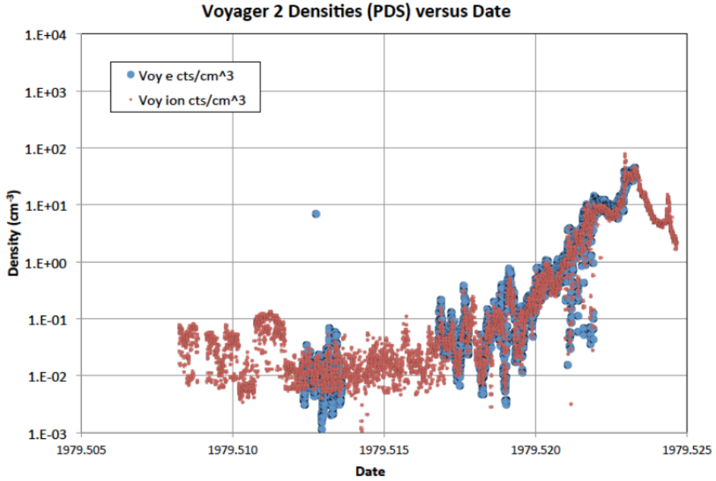
Figure 7. Voyager 2 electron and ion density observations versus time during the flyby of Jupiter. The data (“Voy e cts/cm 3 ” and “Voy ion cts/cm 3 ”) are taken directly from the PDS.
