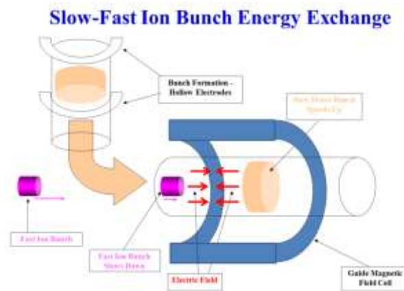
Figure 3.2.1-1- Conceptual scheme for fast to slow bunch interaction
