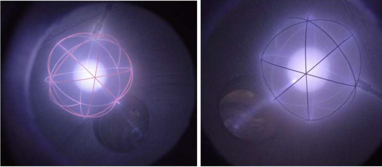
Figure 3.5.1-3. IEC Device at UIUC: IEC plasma with energized grid and formation of plasma jet
