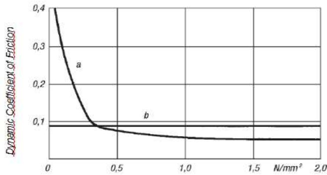
Figure 4.1 Dynamic friction of Polytetrafluoroethylene (PTFE) „Virginal Rundstäbe“ manufactured by Polytetra Moenchengladbach/Germany. Line a: Standard PTFE, line b: Fibreglass enhanced PTFE (Dominghaus, 2007)
