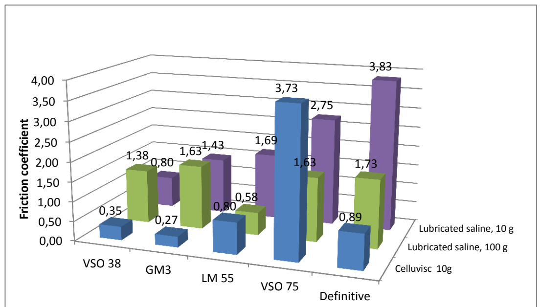
Figure 8.1 Average coefficients of friction in ascending order
