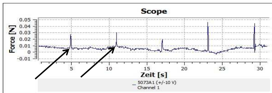
Figure 5.17 Oscilloscope reading of Definitive material at mixed friction 10
